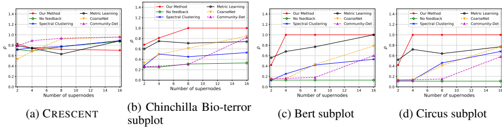
Figure 2: Quality of summaries in (a) CRESCENT and (b-d) different subplots of the VAST 2007 dataset. Note, NetReAct generates network summaries with the highest \rho .
