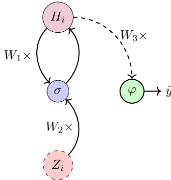
Figure 2: A diagram of a recurrent neural network for a binary classification task.
