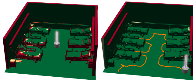
Fig. 1: Comparison of a standard stationary mobile robot (left) against an optimized motion (right). Robot carries a tower light. Surfaces are color coded by UV fluence received, with red indicating 0 \text{ J/m}^2 and green indicating 280 \text{ J/m}^2 or higher. A stationary light cannot to disinfect much of the environment after 30 minutes, while a mobile robot following our optimally computed trajectory (in orange) achieves near complete coverage. (Best seen in color)
