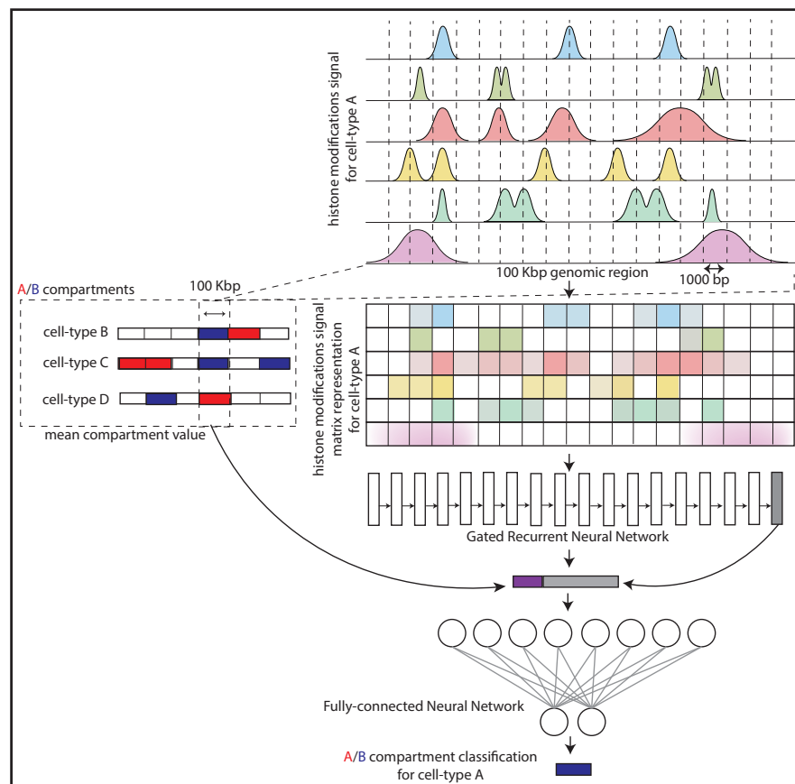
Figure 2. CoRNN architecture: The main input into the model is a matrix X \in \mathbb{R}^{m \times t} . Here, m = 6 denotes the number of histone marks, and t = 100 are the number of genomic bins representing a 100kbp genomic region. The model consists of gated recurrent unit (GRU) layers to capture the sequential information of the histone modification signals across the genomic region. The output of the GRU is then concatenated with the mean compartment value c for the training cell lines and fed into fully connected layers. The output y \in [0, 1] represents the binarized compartment value for the input genomic region.
