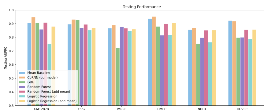
Figure 12. Testing results of CoRNN and baselines using AUPRC score. Our model outperforms the mean baseline for five out of six cell lines
