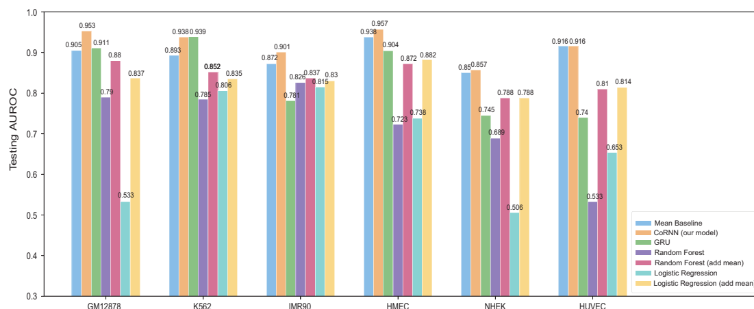
Figure 3. Testing results of CoRNN and baselines. Our model gives the best prediction performance across all cell lines and outperforms the mean baseline for five out of six cell lines.
