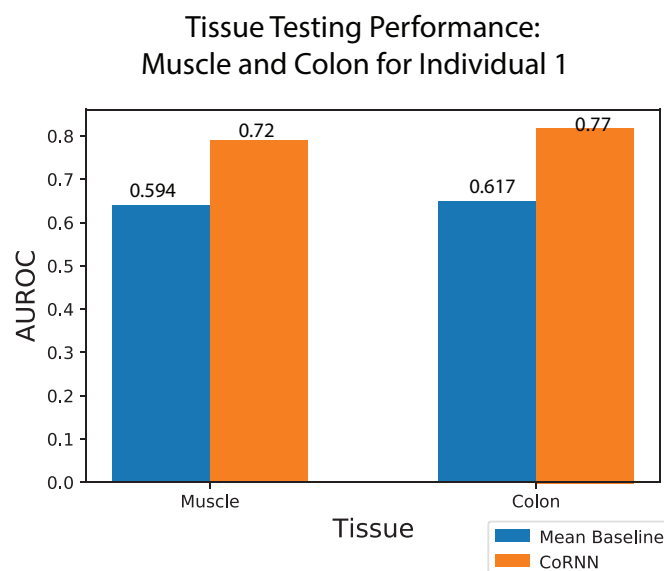
Figure 7. Testing CoRNN and mean baseline on human muscle and colon tissue samples. CoRNN predicts A/B compartments for both tissues with higher AUROC scores compare to mean baseline.
