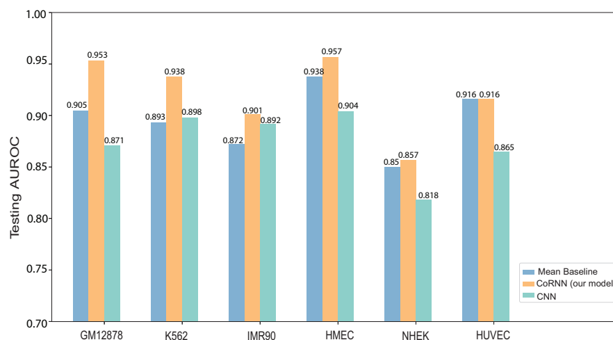
Figure 8. Testing results of CoRNN and Convolutional neural network model. Our model outperforms the convolutional neural network, thus justifying the choice of GRU as our neural network architecture.
