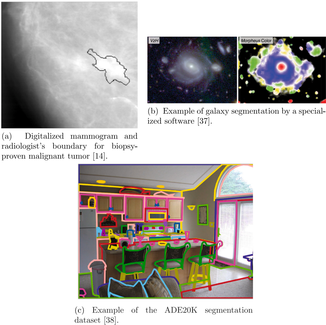
Fig. 2. Medical and astronomical study with direct application of the semantic segmentation task. These images and metallographs have in common a local characteristic. This differentiates them from typical segmentation benchmark datasets such as Cityscapes [39] or ADE20K [38] (on Fig. 2c), where a global scene gives structure to the image. Moreover, unlike the usual benchmark datasets, the annotation can be performed exclusively by experts in the area. This adds an additional difficulty to the problem.
