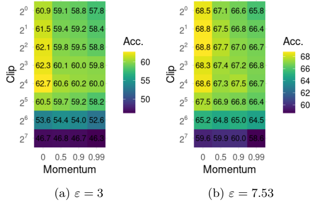
Figure 11: Accuracy (%) under different combinations of clipping bound and first order momentum. The network is DP-CNN and the optimizer is Adam (Kingma & Ba, 2014).
