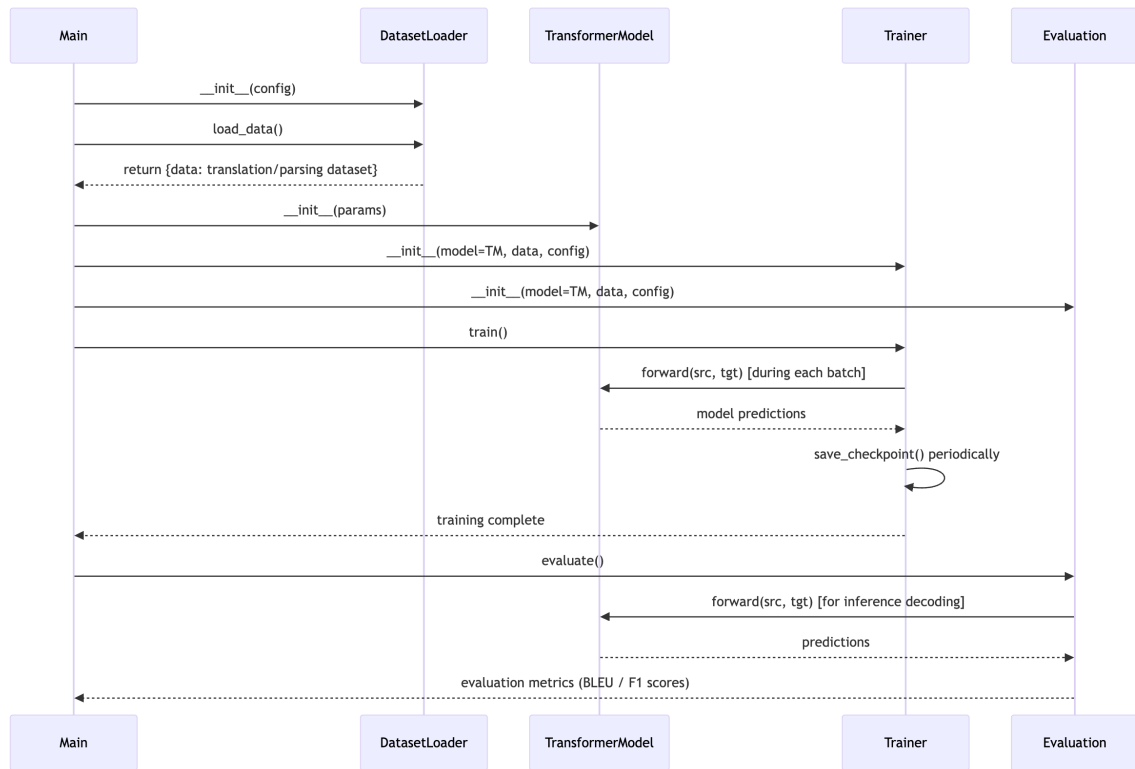
Figure 33: Program call flow visualization generated from Step 1.2 (Architecture Design) in the planning stage of PaperCoder, generated during repository construction for the Transformer [43].
