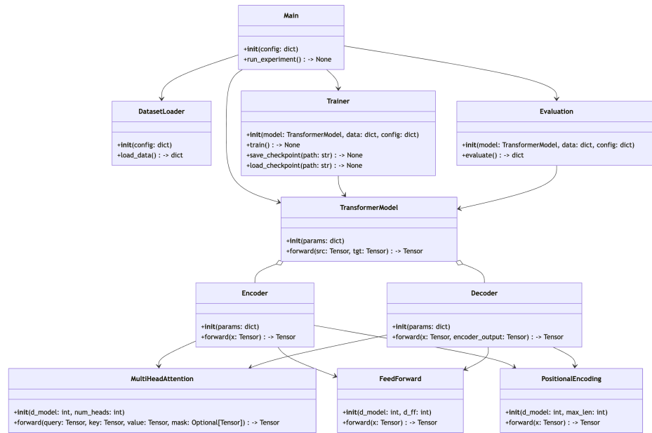
Figure 32: Class diagram visualization generated from Step 1.2 (Architecture Design) in the planning stage of PaperCoder, generated during repository construction for the Transformer [43].
