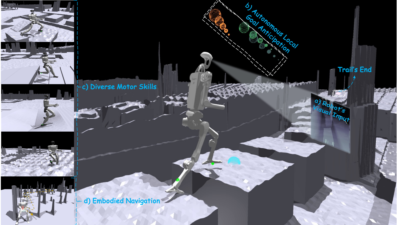
Fig. 1: We propose training humanoids to hike complex trails, driving integrative skill development across visual perception, decision-making, and motor execution. Center: The humanoid robot (H1) a) equipped with vision, learns to b) anticipate near-future local goals to guide locomotion along the trail with self-autonomy. Bubble size (large \rightarrow small) indicates anticipated goal direction; color shows temporal order (orange \rightarrow green \rightarrow forest). Left: Our LEGO-H framework is universal to different humanoid robots (e.g., G1, a smaller robot) to adaptively c) emerge diverse motor skills, and d) develop embodied path exploration strategies to hike on trails with varied terrains and obstacles.
