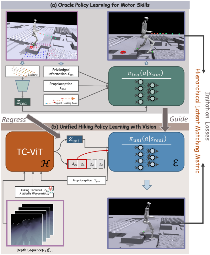
Fig. 2: LEGO-H framework overview. LEGO-H equips humanoid robots with adaptive hiking skills by integrating navigation \mathcal{H} and locomotion \mathcal{E} in a unified, end-to-end learning framework (b). To foster the versatility of motor skills, we train the unified policy via privileged learning from the oracle policy (a).
