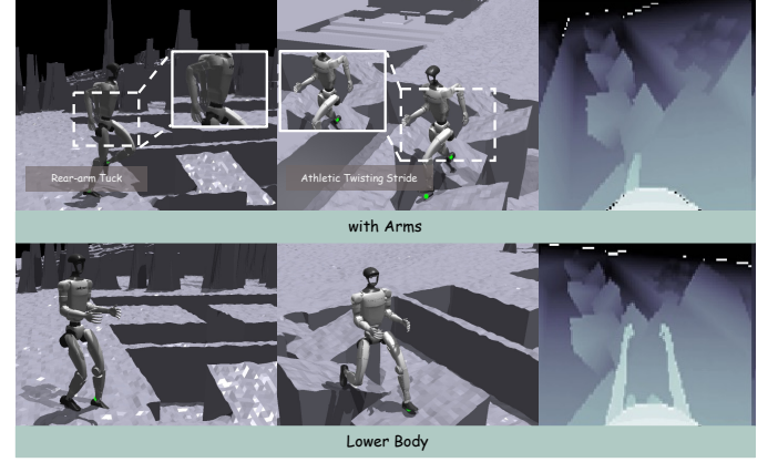
Fig. 9: Preliminary observations for future work on WBC setting. G1 exhibits distinct motor behaviors over with arms vs only lower body . Besides, G1 emerges a rear-arm tuck posture while walking, likely to minimize arm interference with vision (see depth map).
