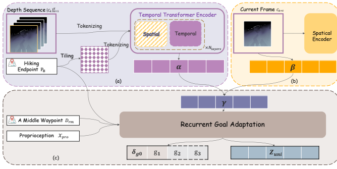
Fig. 3: TC-ViT Architecture. Three key components: a) a goal-orientated temporal transformer encoder for robots cognizing surroundings with the final goal; b) a parallel process on the current depth frame for integrating spatially precise information to reflect the current state c) a recurrent goal adaptation mechanism that integrates visual awareness, goal information, and proprioception.
