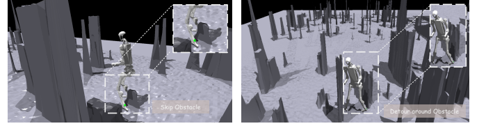
Fig. 6: Navigation in diverse situations. Robots developed different navigation skills, such as directly skipping a small obstacle and detouring around a high obstacle to edge through.
