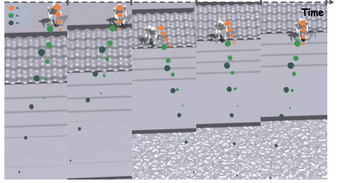
Fig. 4: Dynamic adjustments of near goal anticipation. Snapshots from left to right show a robot traversing mixed terrains along a trail. TC-ViT does not provide a fixed trajectory that locomotion module must rigidly follow. Instead, it predicts several near-future goals ( g_1, g_2, g_3 ), which dynamically adapt to robot’s current state, reflecting real-time adjustments to its navigation decisions. Bubble size (large \rightarrow small) represents predicted local navigation direction.
