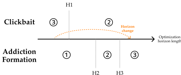
Figure 11. Changing the horizon might make a kind of influence suboptimal but render other kinds of influences optimal. The figure displays a hypothetical situation in which increasing the horizon in order to reduce clickbait enables the system to discover addiction formation strategies. The circled numbers follow the same scheme as in Figure 9.
