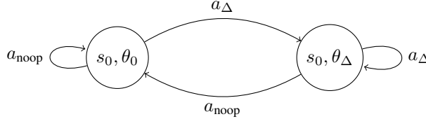
Figure 12. A simple DR-MDP which can lead U_{\text{RT}} to lead certain actions to be optimal that all reward functions disagree with.
