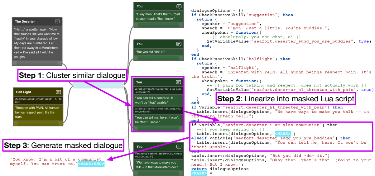
Figure 2: In this conversation from Disco Elysium: The Final Cut , we first cluster dialogue nodes by semantic similarity of game state variables and spoken dialogue. Then, we linearize the next turn of dialogue in the graph into a Lua script that contains game logic and dialogue. Finally, we <MASK> one utterance from the cluster and ask GPT-4 (an LLM trained on code and natural language) to infill the masked dialogue.
