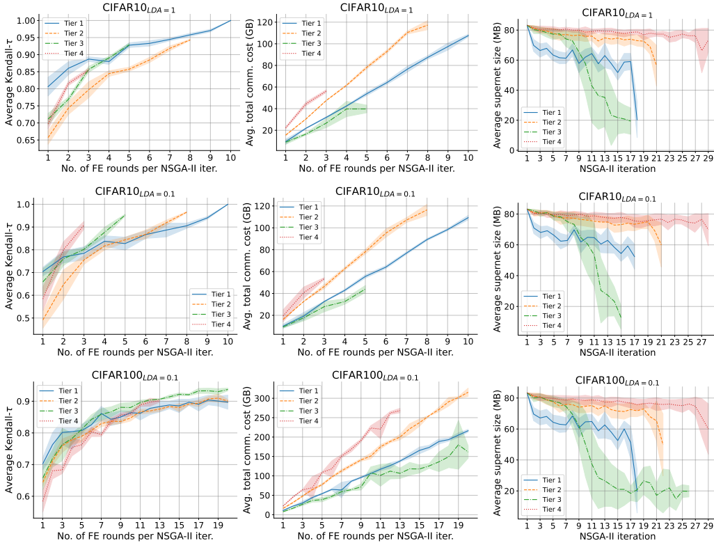
Figure 11: Ranking quality & cost of federated evaluation (FE) of models during federated search. Each time a new population of models is evaluated, a minimal supernet encompassing selected models is sent to a sample of clients; left) ranking correlation between scores produced by FE & centralised evaluation (CE), as a function of FE rounds ( \uparrow rounds = \uparrow clients); middle) total communication cost of sending all necessary supernets to all clients, to run a full search; right) changes in the supernet size as NSGA-II progresses.
