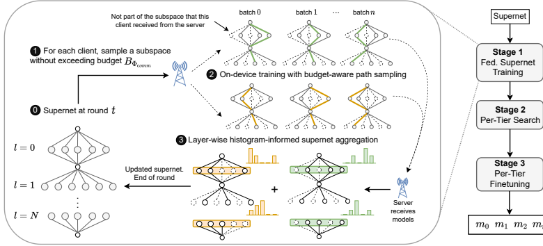
Figure 2: Training process workflow with FedorAS.
