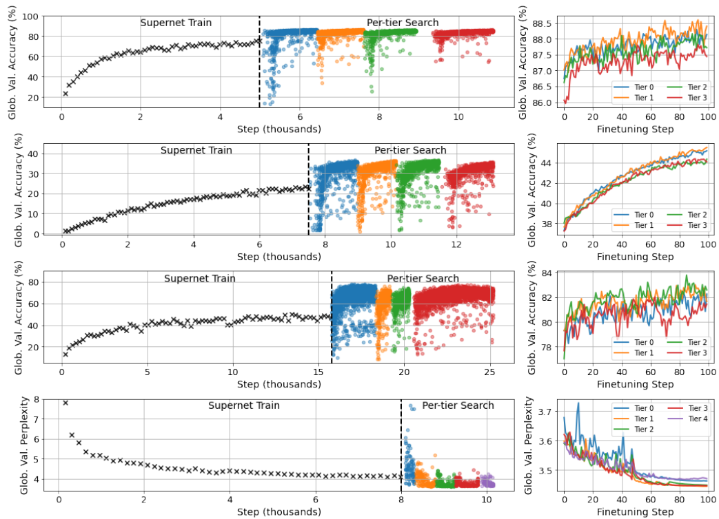
Figure 9: Convergence analysis for each of the datasets considered in this work (from top to bottom: CIFAR-10, CIFAR-100, Speech Commands and, Shakespear). For each dataset, the three stages in FedorAS are shown in the first subplot in the row (Stages I&II) and the subplot on the right shows the final per-tier finetuning (Stage III). Per-tier search and finetuning is colour-coded.
