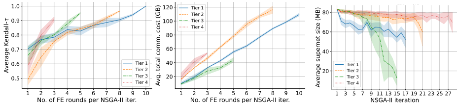
Figure 4: Ranking quality & cost of federated evaluation (FE) of models for CIFAR-10 _{\alpha=0.1} during federated search. Each time a new population of models is evaluated, a minimal supernet encompassing selected models is sent to a sample of clients: left ) ranking correlation between scores produced by FE & centralised evaluation (CE), as a function of FE rounds ( \uparrow rounds = \uparrow clients); middle ) total communication cost of sending all necessary supernets to all clients, to run a full search; right ) changes in the supernet size as NSGA-II progresses.
