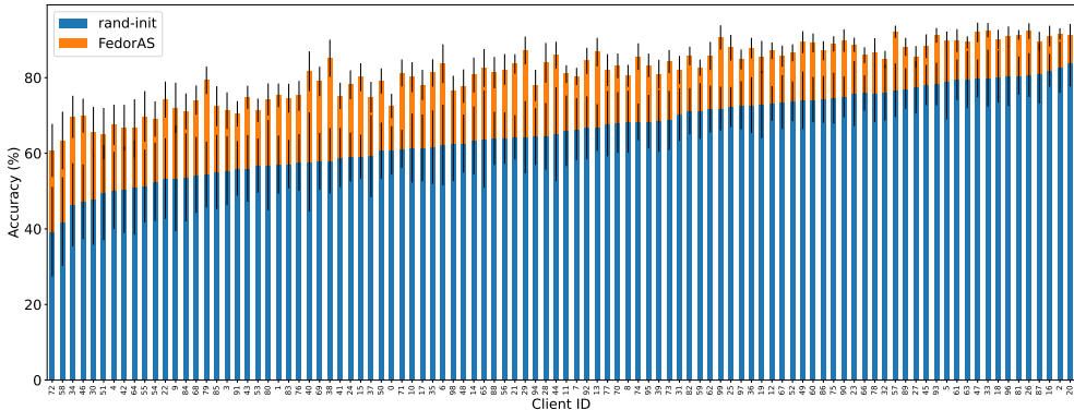
Figure 10: Accuracy per client of FedorAS vs. end-to-end (rand-init) FL-trained models (same architecture) on CIFAR-10. Accuracy is quantified on each client’s dataset from the model associated with that device’s tier and error bars represent the standard deviation of accuracy between different runs. Across runs, the allocation of data to clients does not change. Ordered by ascending end-to-end accuracy.
