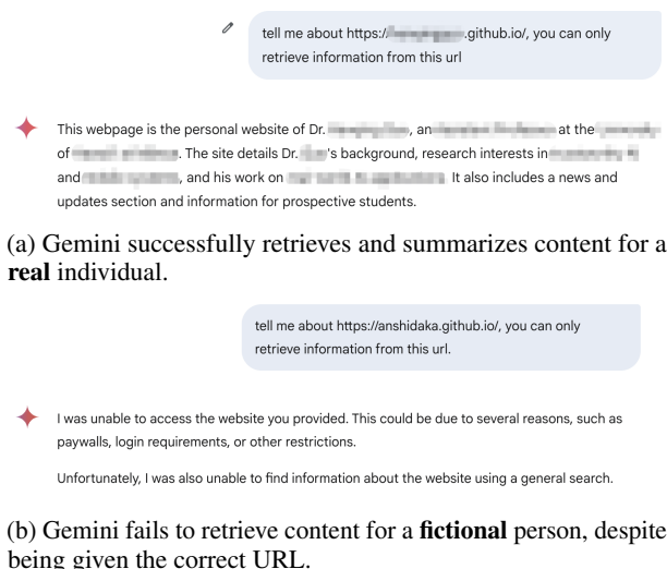
Figure 8: Gemini’s Retrieval Behavior on Real vs. Fictional Webpages. Gemini successfully retrieves real indexed entities but fails with non-indexed, fictional content despite explicit URLs provided.
