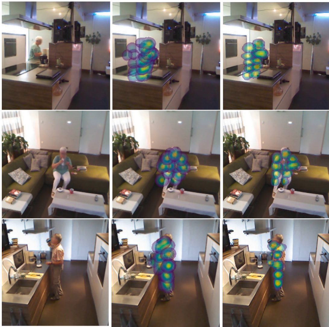
Fig. 10. Sample heatmaps from the Toyota-SmartHome (CS) dataset test set using PO-GUISE. The first column corresponds to the middle frame of the video clip, the second column displays the temporal heatmaps used as training labels, and the third column shows the predicted heatmaps.
