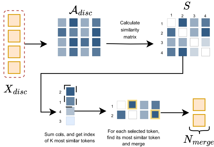
Fig. 5. Token merging diagram. The discarded tokens from the previous pruning step are merged by their similarity. The similarity between tokens is measured by their attention to each other ( A_{disc} ). The N_{merge} most similar tokens are selected and then merged with their corresponding most similar token.
