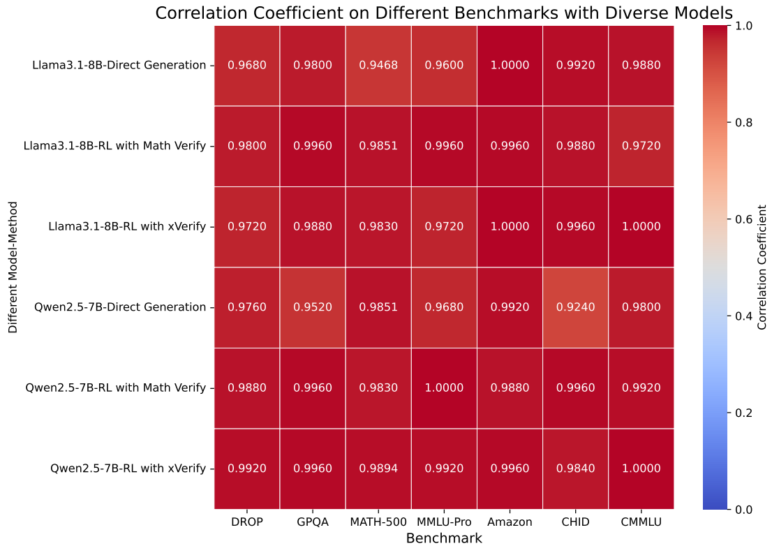
Figure 21: The Consistency between xVerify and Human Evaluation
