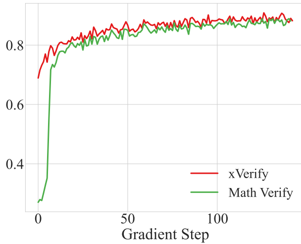
Figure 23: Learning Curves of Llama3.1-8B in Reinforcement Learning
