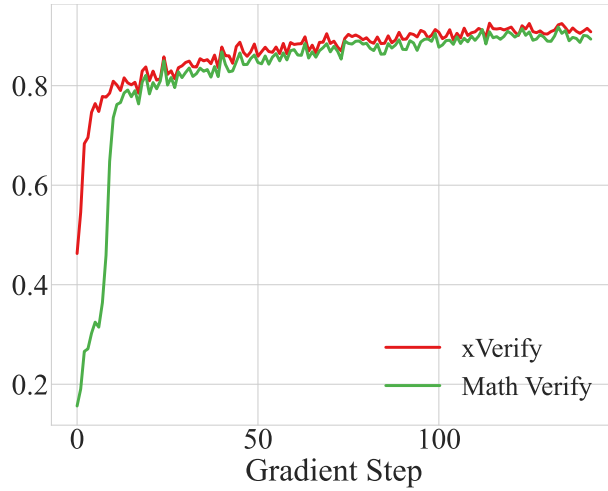
Figure 22: Learning Curves of Qwen2.5-7B in Reinforcement Learning
