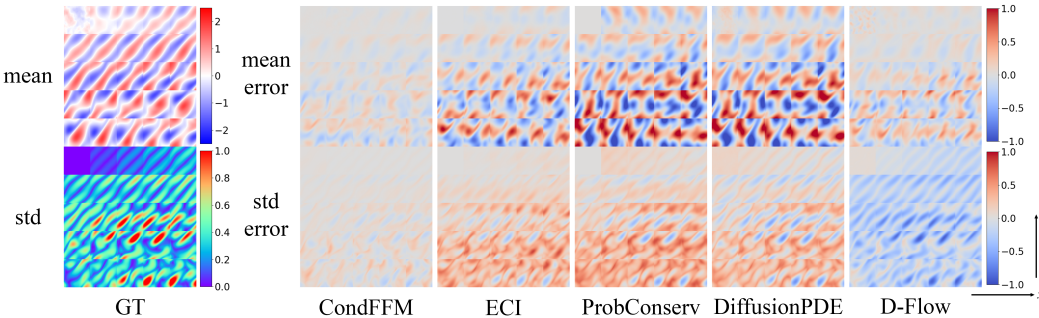
Figure 3: Generation mean and standard deviation errors of the trajectories for the NS equation with IC fixed. 25 downsampled time frames are plotted for each method.
