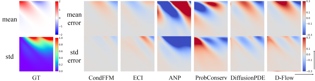
Figure 2: Generation mean and standard deviation errors for the Stokes problem with IC fixed. Note that grey indicates \approx 0 error, red for positive error, and blue for negative error. Noticeable IC errors (left column) can be observed for the gradient-based methods.
