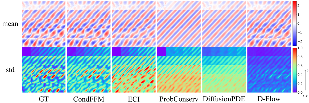
Figure 15: Generation mean and standard deviation for the 2D NS equation with IC fixed.
