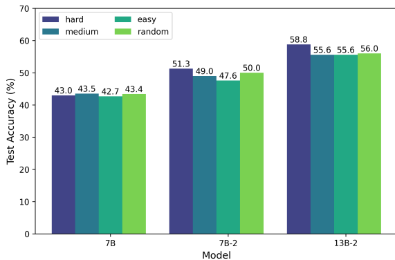
Figure 5: The performance of SFT models with different difficulty augmentation on GSM8K.
