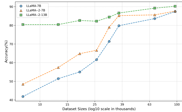
Figure 7: The relationship of accuracy on the training set and the amounts of augmentation data.
