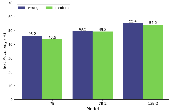
Figure 6: The performance of SFT models with wrong problem augmentation on GSM8K.
