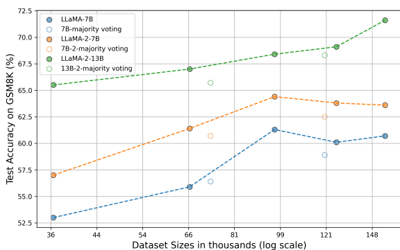
Figure 3: Comparison of test set accuracy on GSM8K for models of varying scales after fine-tuning on AugGSM8K subsets with different response augmentation amount.
