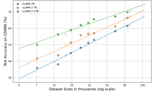
Figure 2: Comparison of test set accuracy on GSM8K for models of varying scales after fine-tuning on AugGSM8K subsets with different query augmentation amount.
