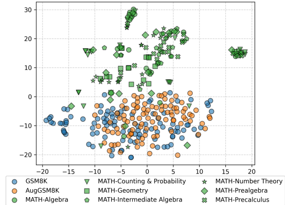
Figure 4: The embedding visualization of queries in GSM8K, MATH and AugGSM8K.
