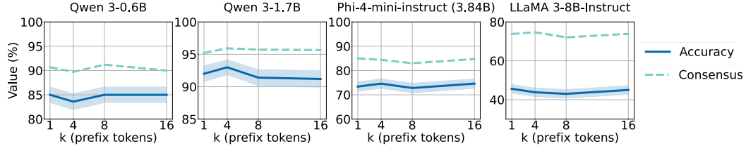
Figure 5: Two-agent THOUGHTCOMM with accuracy (solid) and consensus (dashed) performance on MATH [Hendrycks et al., 2021] as prefix length increases from 1 to 16.
