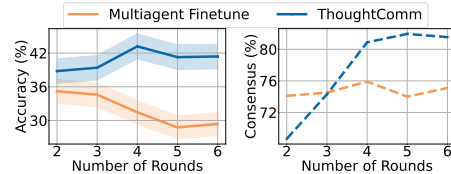
Figure 6: Multi-agent performance as the number of debate rounds increases.
