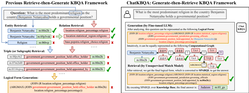
Figure 1: Comparison of examples of the previous retrieve-then-generate KBQA framework (left) and our proposed generate-then-retrieve KBQA framework, ChatKBQA (right). Note that labels such as “g.g.a” etc. in the computational graph are acronyms for relation names such as “government.government.position.held.appointed.by”.
