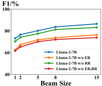
Figure 4: Ablation study in ChatKBQA retrieval phase to verify the effectiveness of Beam Search, Entity Retrieval (ER), and Relation Retrieval (RR), respectively.
