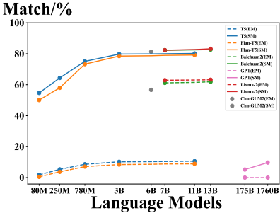
Figure 5: Comparison with other LMs in ChatKBQA generation phase.
