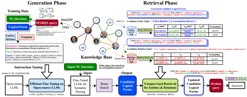
Figure 2: The overview of ChatKBQA framework for generate-then-retrieve KBQA method with fine-tuned LLMs and unsupervised retrieval for entities and relations in candidate logical forms.
