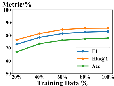
Figure 3: Ablation study in ChatKBQA generation phase to verify the effectiveness of LLM’s Fine-tuning.
