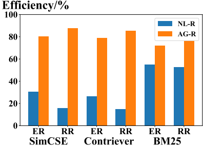
Figure 6: Comparison of retrieval efficiency between retrieval from nature language questions (NL-R) and generated logical forms (AG-R) in ChatKBQA retrieval phase.
