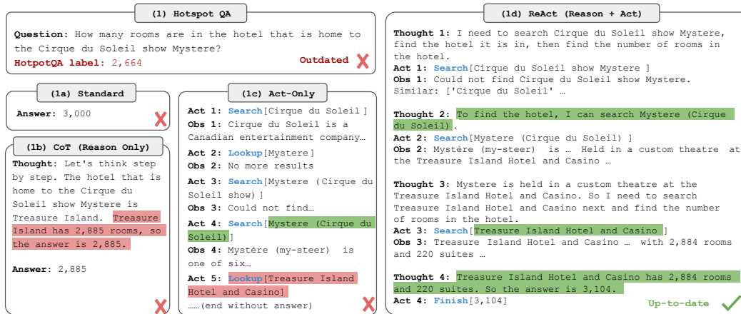
Figure 5: Another example HotspotQA question, where the original label is outdated. Only ReAct is able to obtain the up-to-date answer thanks to real-world web interaction plus reasoning.
