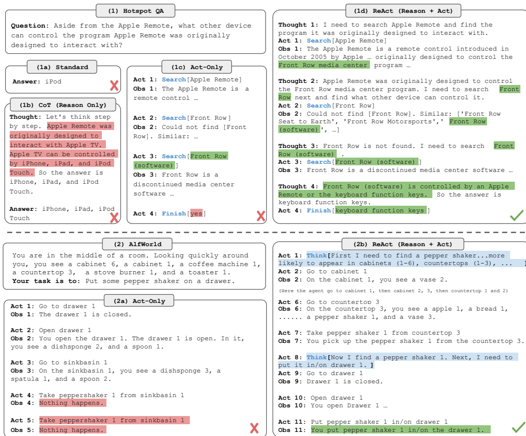
Figure 1: (1) Comparison of four prompting methods, (a) Standard, (b) Chain-of-thought (CoT, Reason Only), (c) Act-only, and (d) ReAct (Reason+Act), solving a HotspotQA (Yang et al., 2018) question. (2) Comparison of (a) Act-only and (b) ReAct prompting methods to solve an interactive AlfWorld (Shridhar et al., 2020b) task. In both domains, we omit initial prompts of in-context examples, and only show task solving trajectories generated by the model (Act, Thought) and the environment (Obs).
