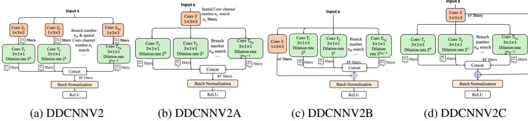
Figure 3: Illustration of the search blocks for the first six blocks in the AutoShot. It consists of four types of factorized 3D convolution blocks, (a) DDCNNV2 with 2D spatial convolutions followed by 1D temporal convolutions, (b) DDCNNV2A with a shared 2D spatial convolution and 1D temporal convolutions, (c) DDCNNV2B accumulating a 2D spatial convolution and 1D temporal convolutions, and (d) DDCNNV2C compromising between DDCNNV2A and DDCNNV2B.
