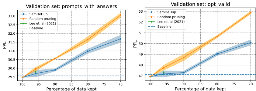
Figure A7: SemDeDup applied to C4 . The x-axis corresponds to different percents of data kept, and the y-axis represents the perplexity on validation sets described in Section D.1 (lower is better). Each point is a separate 125M model trained on one-pass of its respective pruned dataset (mean and standard deviation across 3 random training seeds). The green point represents a 125M model trained on a version of C4 deduplicated via the NearDup method (Lee et al., 2021a). Note that NearDup (the single green point) keeps 96.1% of the data. SemDeDup can match this baseline performance while keeping only 80% of the data (see Table A17 for numerical comparison).
