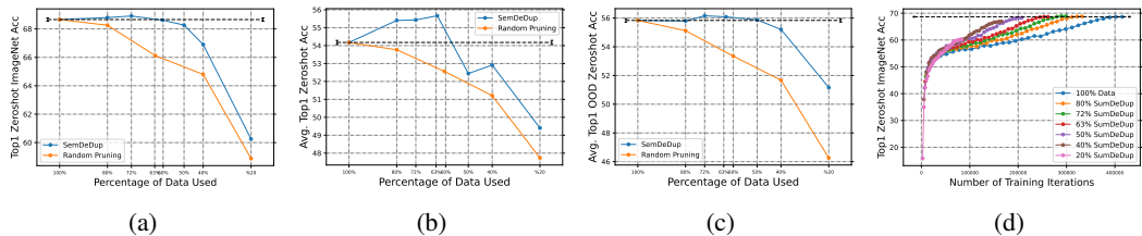
Figure 3: SemDeDup allows better average zero-shot accuracy across 30 tasks with less data and faster pre-training. (a): Down to using only 50% of LAION-440M for pre-training CLIP, we are able match the zero-shot ImageNet accuracy of the baseline model trained on 100% of the data (black dashed line) with a small drop of 0.38% only, while we outperform the baseline model with only 63% of data. (b): Average zero-shot performance for CLIP measured on 24 datasets improves down to 63% of the pre-training data, yielding better performance with almost 1.6\times faster pre-training. (c): Zeroshot validation accuracy averaged over 6 ImageNet-1k OOD datasets. (d): We track zeroshot ImageNet-1K performance as a function of LAION-440M pre-training iterations at different deduplication thresholds. With SemDeDup, models converge in far less iterations. The black dashed line corresponds to the average performance over 4 different training seeds for a baseline model trained on 100% of the data. The error bars indicate the standard deviation (std) of performance.
