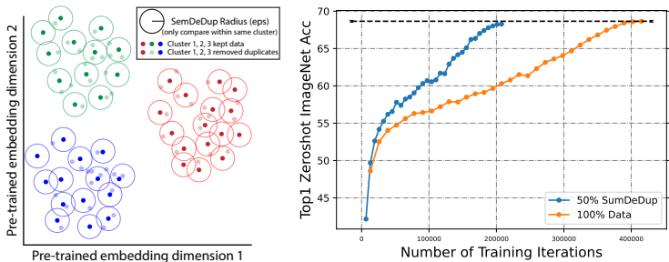
Figure 1: Data efficiency from semantic deduplication (SemDeDup) (left): A schematic of the SemDeDup algorithm which efficiently removes semantic duplicates from web-scale data. (right): When SemDeDup removes 50% of the LAION-440M dataset, training on this semantically nonredundant subset achieves almost the same performance as training on the entire 440M dataset. Also, training speed is twice as fast and completes in half the time.
