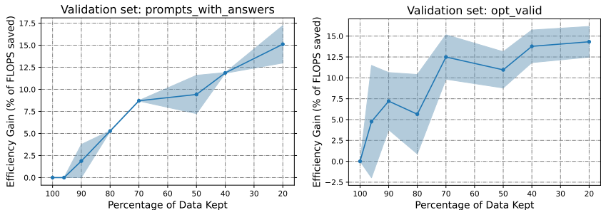
Figure A8: SemDeDup allows compute efficiency gains by training on much smaller datasets for slightly longer . We prune datasets via SemDeDup and continue training past one epoch until we reach baseline model perplexity. The x-axis is the percentage of data kept, and the y-axis is the percentage of FLOPs saved. For example, training on the 80% pruned dataset reaches baseline model perplexity on prompts_with_answer in 95.0% of the baseline training, saving 5.0% compute. Mean and standard deviation provided across 3 random training seeds.
