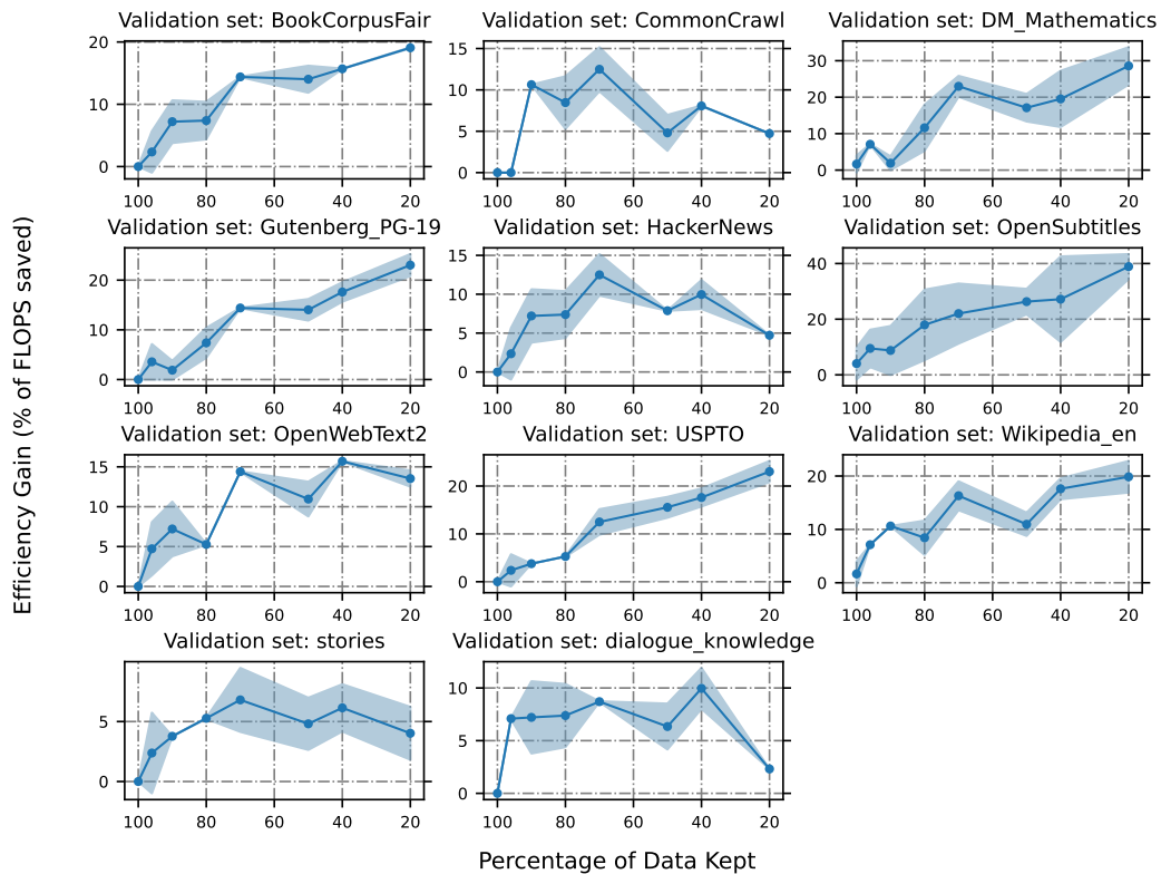
Figure A25: Percentage of Data Kept vs. Efficiency Gain on individual validation sets within opt_valid . Runs are averaged across training seeds where the model achieves baseline perplexity at some point in training, and shaded regions represent 1 standard deviation from the mean. The title of each plot represents the name of the individual validation set within opt_valid .
