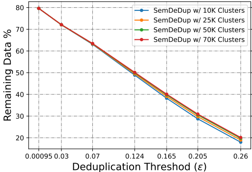
Figure A10: Deduplicated dataset size as a function of the deduplication threshold for different values of k-means clusters k . Note that the range in the resulting deduplicated dataset size is 0.003% when \epsilon is 0.00095 and 2% when \epsilon is 0.26.
