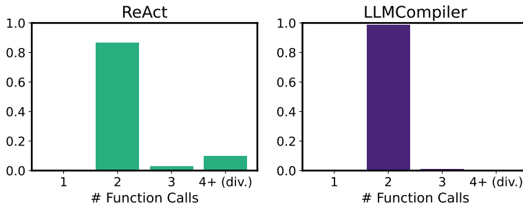
Figure A.3. Distributions of the number of function calls when running the HotpotQA benchmark on ReAct (Left) and LLMCompiler (Right). While LLMCompiler (Right) consistently completes the task within 2 function calls, which is expected as HotpotQA exhibits a 2-way parallelizable pattern, ReAct (Left) shows that around 10% of the examples undergo repetitive (>4) function calls, resulting in a diverging behavior of the framework. LLaMA-2 70B is used for the experiment.
