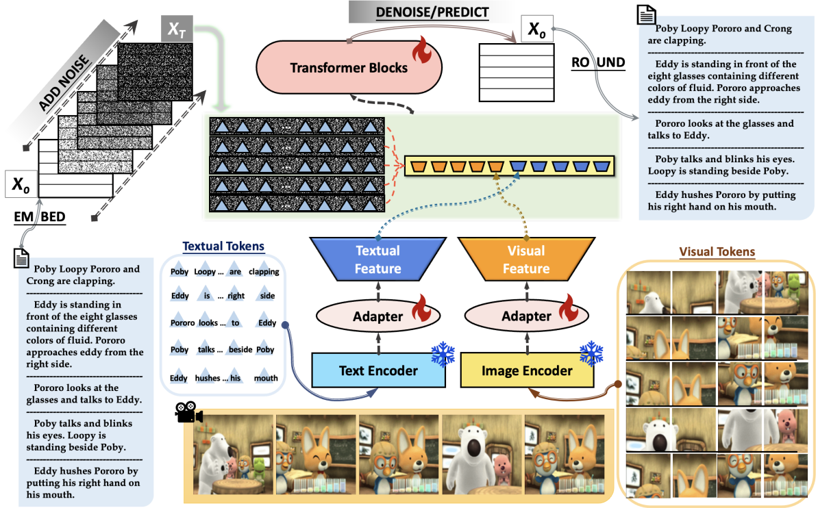
Figure 2: Overview of DIFFUVST: First, two pretrained encoders extract the image- and text features of all panels of the story, which are then transferred to the current dataset domain via trainable adapter modules. Next, these feature segments are fused into the corrupted word embeddings x_T to provide global history condition (image) and classifier-free guidance (text) across the entire picture stream. Finally, a transformer learns to restore the word embeddings of the story ( x_0 ) from the fused vector input, which can be grounded back to the actual text.
