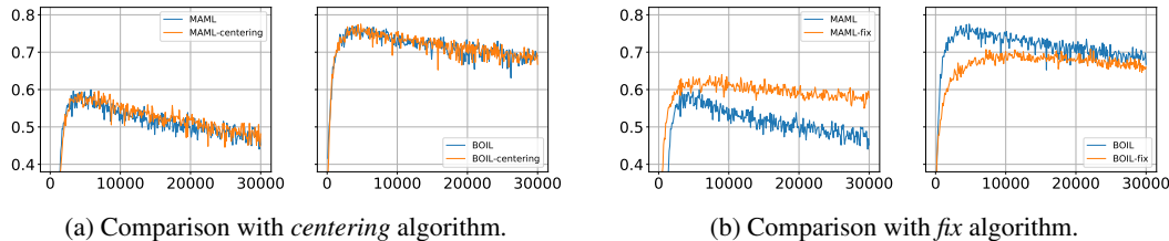
Figure 20: Valid accuracy curves of (a) centering algorithm and (b) fix algorithm on Cars.
