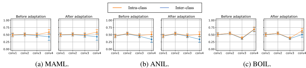
Figure 16: Cosine similarity of 4conv network on Cars.
