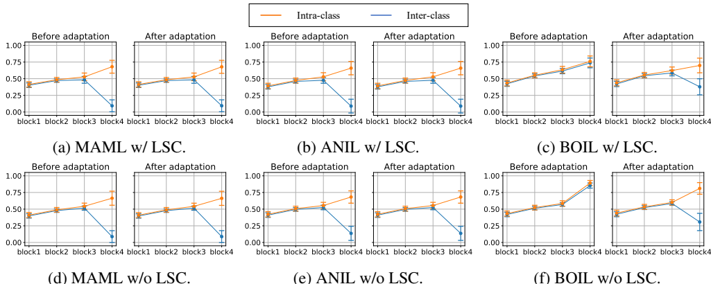
Figure 23: Cosine similarity of ResNet-12 on Cars.
