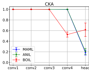
Figure 3: CKA of 4conv.
