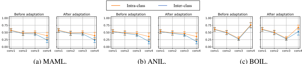
Figure 2: Cosine similarity of 4conv network.
