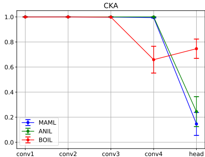
Figure 17: CKA of 4conv on Cars.
