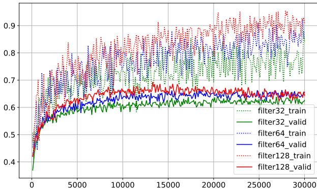
Figure 12: Training/Validation accuracy curve on miniImageNet according to filters in BOIL.
