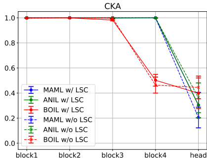
Figure 24: CKA of ResNet-12 on Cars.
