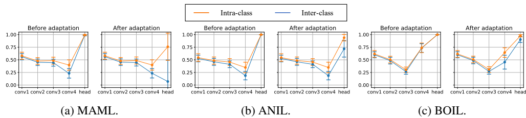
Figure 15: Cosine similarity of 4conv network including head.
