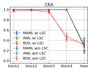
Figure 22: CKA of ResNet-12 on miniImageNet.
