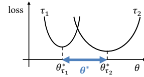
Figure 19: Ideal meta-initialization.
