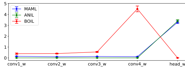
Figure 14: Gradient norm.
