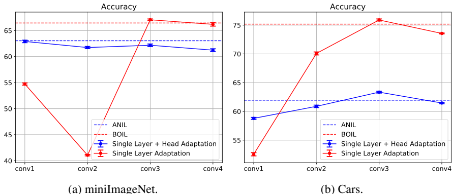
Figure 18: Test accuracy according to the learning layer in the body.
