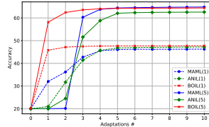
Figure 11: Accuracy on miniImageNet according to the number of adaptation(s).
