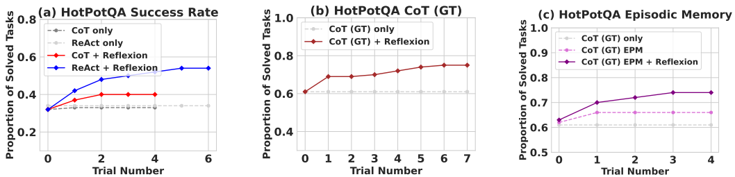
Figure 4: Chain-of-Thought (CoT) and ReAct. Reflexion improves search, information retrieval, and reasoning capabilities on 100 HotPotQA questions. (a) Reflexion ReAct vs Reflexion CoT (b) Reflexion CoT (GT) for reasoning only (c) Reflexion vs episodic memory ablation.
