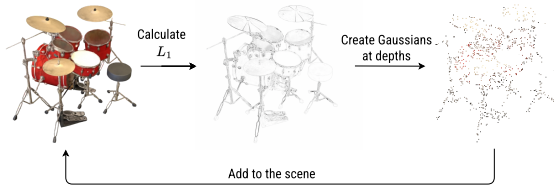
Figure 4. Densification overview. Illustration of the proposed error-guided strategy. We render an image with 3DGS, compute the per-pixel L_1 error, sample pixels proportionally to their error magnitude, and place new Gaussians at the iNGP-predicted depth along the corresponding viewing rays.
