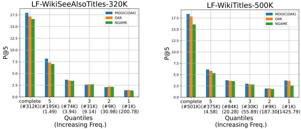
Figure 2: Quantile wise-comparison of MOGIC and other methods for LF-WikiSeeAlsoTitles-320K, LF-WikiTitles-500K
