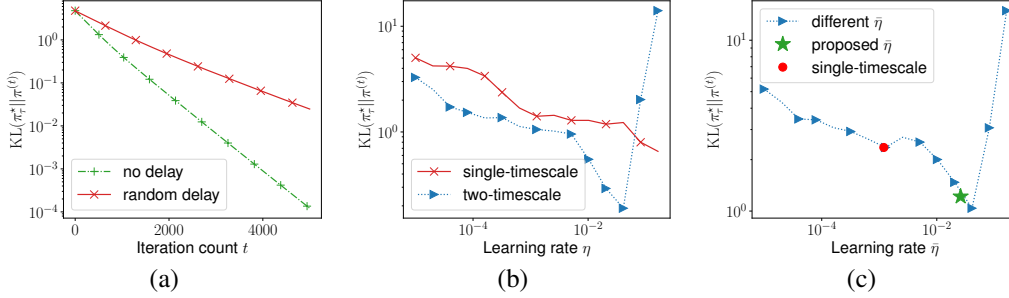
Figure 1: \text{KL}(\pi_\tau^* \parallel \pi^{(t)}) of single-timescale and two-timescale OMWU with respect to different values of learning rate and delay. (a): performance of single-timescale OMWU in the synchronous setting and asynchronous setting. (b) & (c): performance of the two methods after 5000 iterations under various choices of \eta and \bar{\eta} , with \bar{\eta} fixed to \bar{\eta} = \tau^{-1}(1 - (1 - \eta\tau)^{\gamma+1}) in (b) and \eta fixed to 0.001 in (c).
