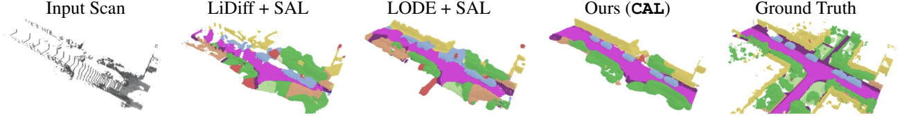
Figure 6. Comparison to zero-shot baselines on SemanticKITTI. Given a single Lidar scan (1 st col.), we compare CAL (4 th col.) to zero-shot baselines (2 nd and 3 rd cols.) combining LiDiff (Nunes et al., 2024) and LODE (Li et al., 2023b) with SAL (Osep et al., 2024).
