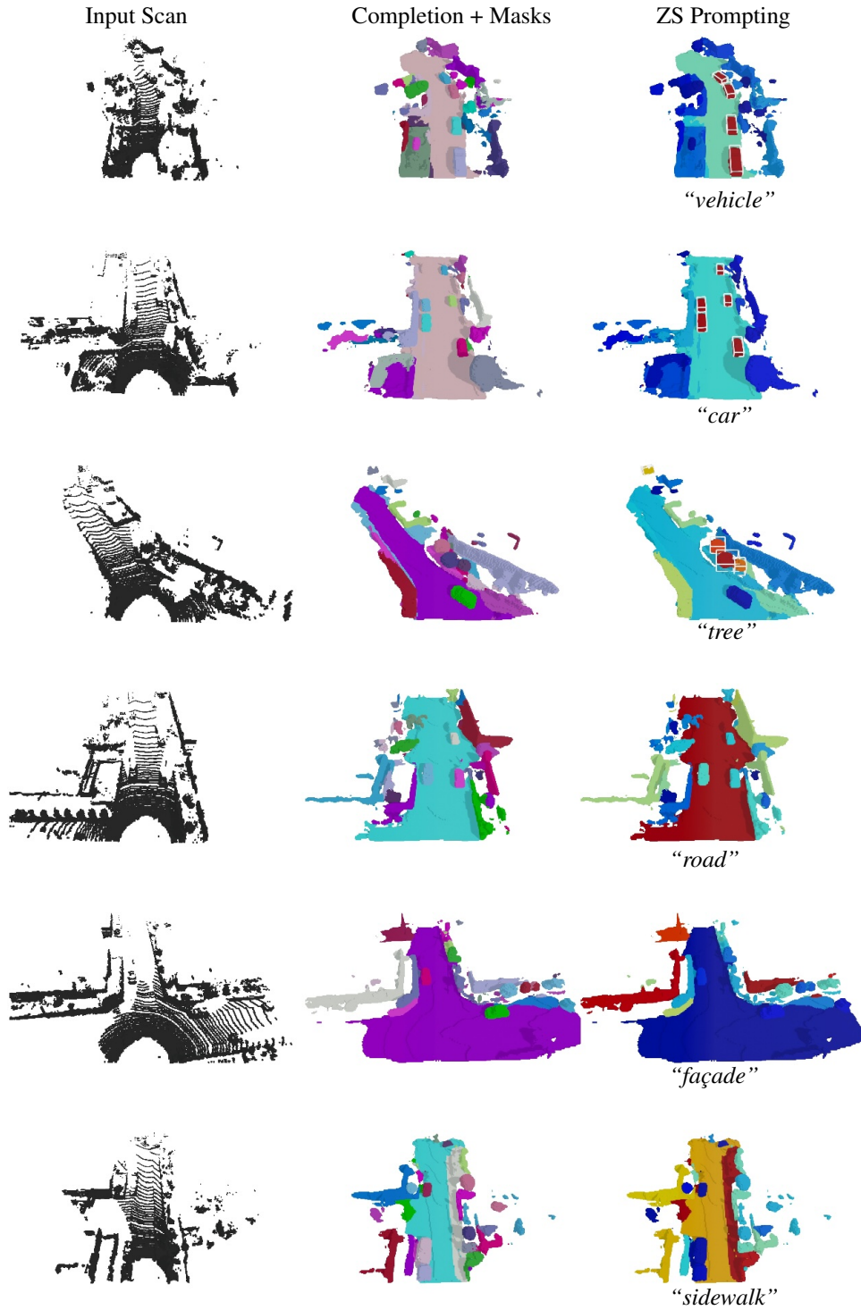
Figure 7. Qualitative results on KITTI-360 (Liao et al., 2021) . Given a single Lidar scan as input (1 st column), CAL completes object-level observations as a set of masks over the voxel grid (2 nd column) with semantic CLIP feature for each predicted mask. We can prompt with any semantic class vocabulary and perform panoptic and semantic scene completion (3 rd column).
