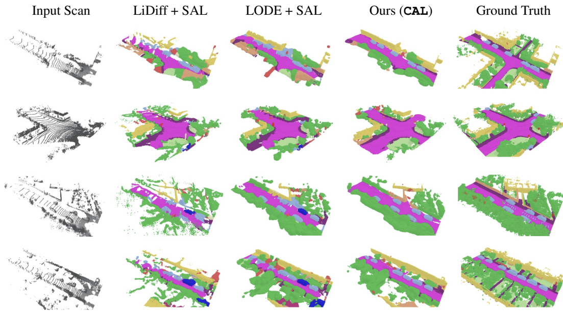
Figure 8. Qualitative comparison to zero-shot baselines on SemanticKITTI. Given a single Lidar scan ( 1^{st} col.), we compare our method ( CAL , 4^{th} col.) to zero-shot baselines ( 2^{nd} and 3^{rd} cols.) combining LiDiff (Nunes et al., 2024) and LODE (Li et al., 2023b) with SAL (Osep et al., 2024). While baselines struggle with coherent structure and semantic accuracy, CAL produces cleaner and more complete outputs that align closely with the ground truth.
