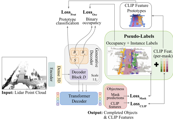
Figure 3. CAL model architecture and training pipeline. The backbone consists of a sparse encoder and a dense 3D convolutional block. We estimate scene-level occupancy using a multi-scale sparse generative decoder that consists of decoder blocks D , two occupancy heads B_o and B_s , and a pseudo-semantic head ( S ) at each scale L . The Transformer decoder then predicts segmentation masks over the completed scene and regresses CLIP features.
