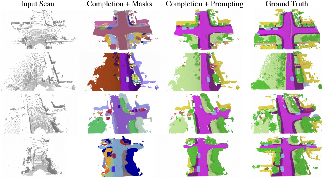
Figure 4. Qualitative results on SemanticKITTI. Given a single Lidar scan (1 st col.), CAL completes object-level observations as a set of masks over the voxel grid (2 nd col.) and predicts a CLIP feature for each mask. We can prompt with any semantic class vocabulary and obtain panoptic and semantic scene completion (3 rd col.) results. Our model predicts shape priors for both thing (e.g., ‘car’, ‘cyclist’) and stuff classes (e.g. ‘vegetation’, ‘road’) and can correctly predict the intersection geometry in 4 th row, despite limited direct evidence.
