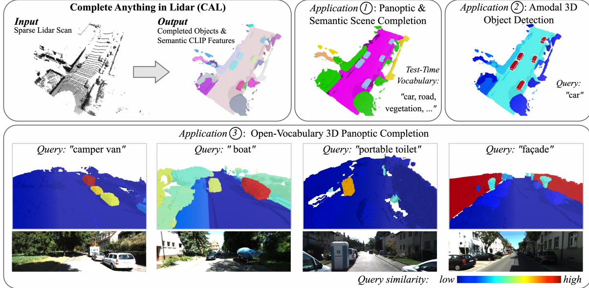
Figure 1. Learning to Complete Anything in Lidar. Given a sparse Lidar point cloud, CAL ( Complete Anything in Lidar ) localizes, reconstructs, and, optionally, recognizes objects in a zero-shot fashion. By providing a semantic class vocabulary of specific object classes at test time, CAL can be prompted to perform Semantic Scene Completion (SSC), Panoptic Scene Completion (PSC), or (amodal) 3D Object Detection. Note that CAL only takes a single Lidar scan as input; RGB images are shown for visualization purposes only.
