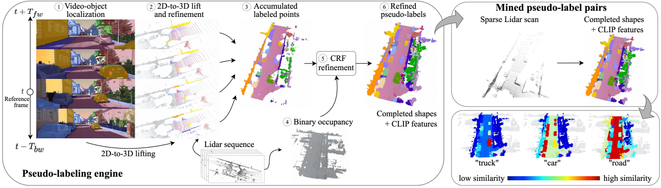
Figure 2. Pseudo-labeling engine. Given a calibrated RGB camera and Lidar sensor, ① we use video-object segmentation models (Ravi et al., 2024) to localize object instances in video, ② pseudo-label the Lidar point clouds over time, and ③ generate completed voxelized object representations, each enriched with a per-instance CLIP feature extracted from RGB images. In ④, we accumulate 360° Lidar scans to obtain full-scene binary occupancy, used for refining the aggregated pseudo-labels ③ via a CRF-guided label refinement process ⑤. As output ⑥, our method pairs each sparse and incomplete Lidar scan with pseudo-labels for object-level scene completion (top-right) and CLIP features, which are temporally aggregated by averaging per-instance features across the sequence. These CLIP features enable zero-shot recognition via text queries (bottom-right). Mined pseudo-label pairs are then used to train the CAL model.
