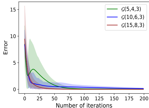
Figure 1. The error of value functions computed by DRPG for three Garnet problems with different sizes.
