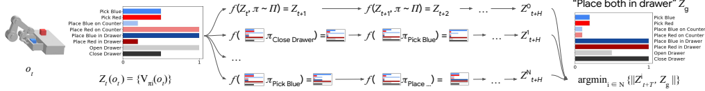
Figure 4: Overview of model-based planning with VFS. We learn a one-step predictive model for the embedding Z_t and use random shooting with a scoring function \epsilon to find the best action to the encoded goal Z_g .
