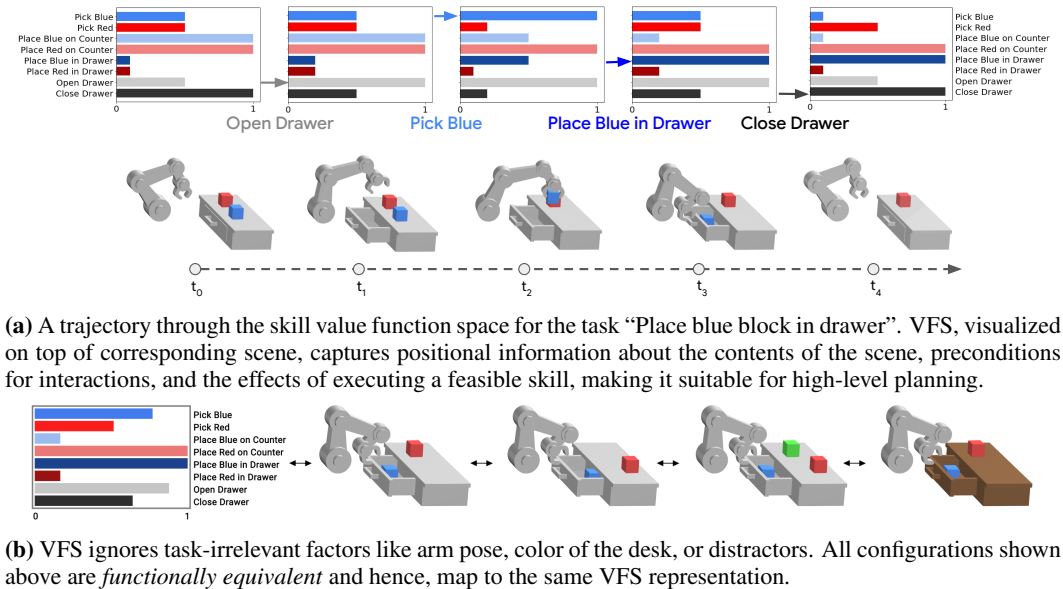
Figure 1: Visualizing VFS embeddings in an example desk rearrangement task. VFS can capture the affordances of the low-level skills while ignoring exogenous distractors.
