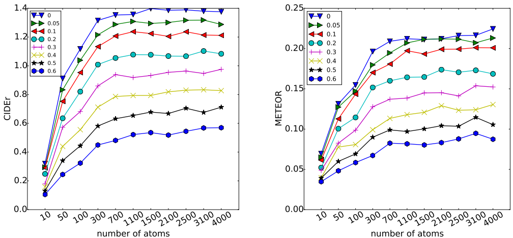
Figure 3: Learned upper bounds with various atom precision on COCO (left) and LSMDC (right). The number of atoms \hat{\mathbf{a}}_r^{(k)} is varied on x-axis and upper bounds are computed on y-axis on testsets. CIDER is used for COCO and METEOR for LSMDC. Compared with Figure 2, the upper bounds are obtained with various atom accuracy ( r in legend) and atom quantity (x-axis). There is a trade-off between atom accuracy and atom quantity. It shows one could increase the score by either improving P(\mathbf{a}^{(k)}|\mathbf{v}) with a fixed k or increase k . It also shows the maximal error bearable for different score.
