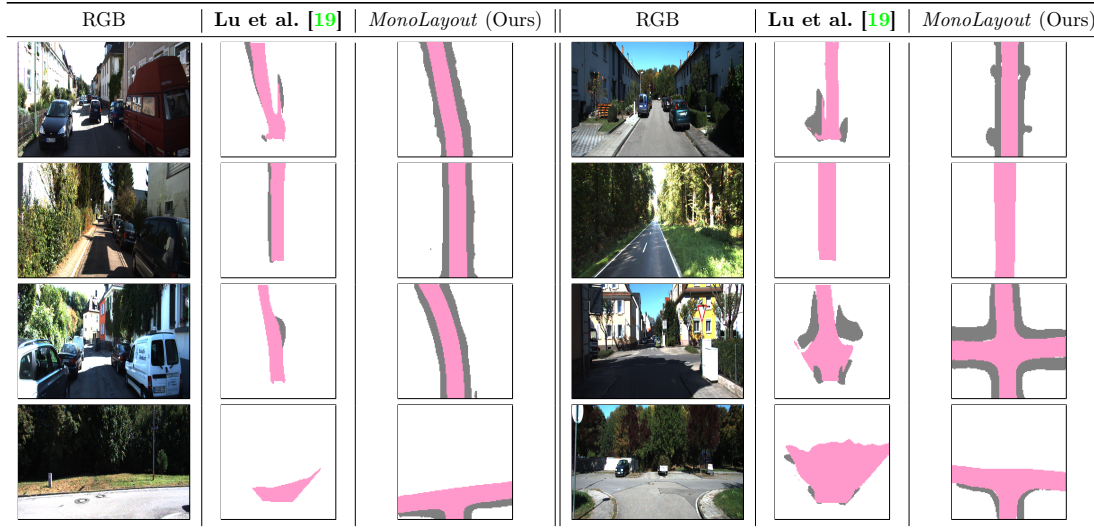
Figure 3: Static layout estimation: Observe how MonoLayout performs amodal completion of the static scene (road shown in pink, sidewalk shown in gray). MonoOccupancy [19] fails to reason beyond occluding objects (top row), and does not hallucinate large missing patches (bottom row), while MonoLayout (Ours) is accurately able to do so. Furthermore, even in cases where there is no occlusion (row 2), MonoLayout (Ours) generates road layouts of much sharper quality. Row 3 show extremely challenging scenarios where most of the view is blocked by vehicles, and the scenes exhibit high-dynamic range (HDR) and shadows.
