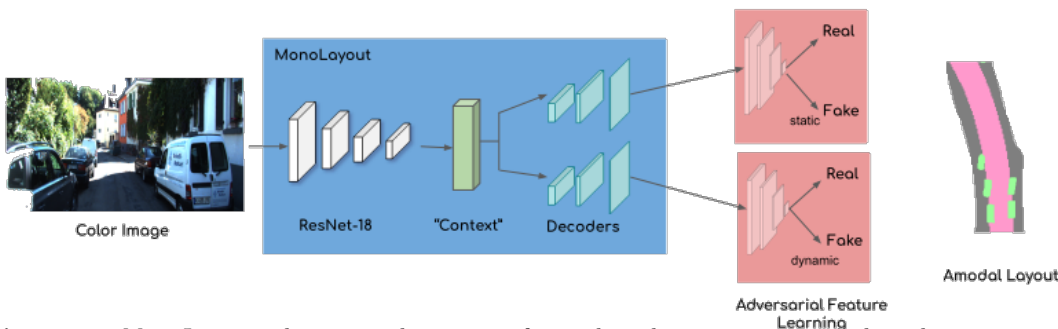
Figure 2: Architecture: MonoLayout takes in a color image of an urban driving scenario, and predicts an amodal scene layout in bird’s eye view. The architecture comprises a context encoder, amodal layout decoders , and two discriminators .
