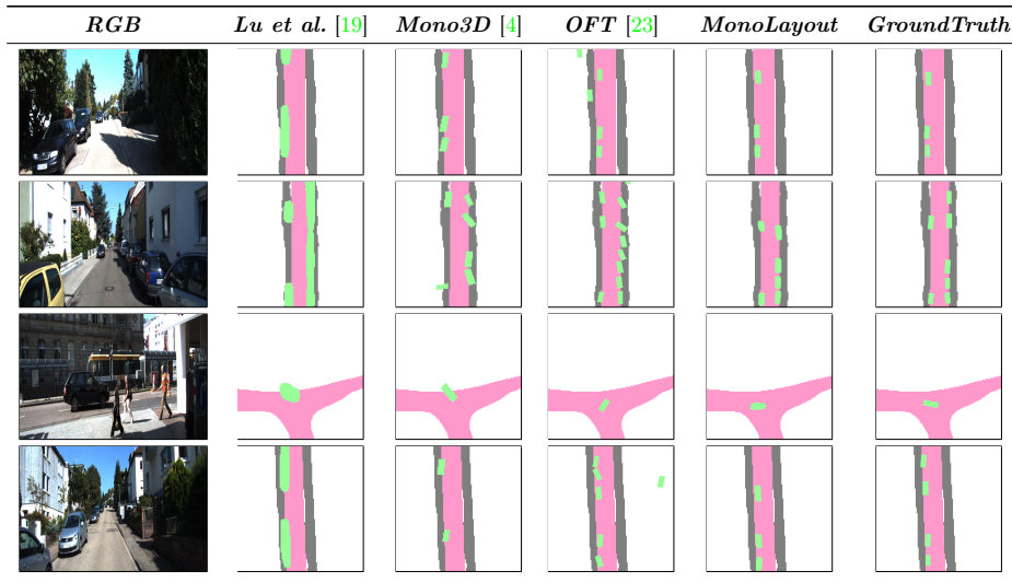
Figure 4: Dynamic layout estimation: We show vehicle occupancy estimation results on the KITTI [8] 3D Object detection benchmark. From left to right, the column corresponds to the input image, MonoOccupancy [19], Mono3D [4], OFT [23], MonoLayout (Ours), and ground-truth respectively. While the other approaches miss out on detecting cars (top row), or split a vehicle detection into two (second row), or stray detections off road (third row), MonoLayout (Ours) produces crisp object boundaries while respecting vehicle and road geometries.
