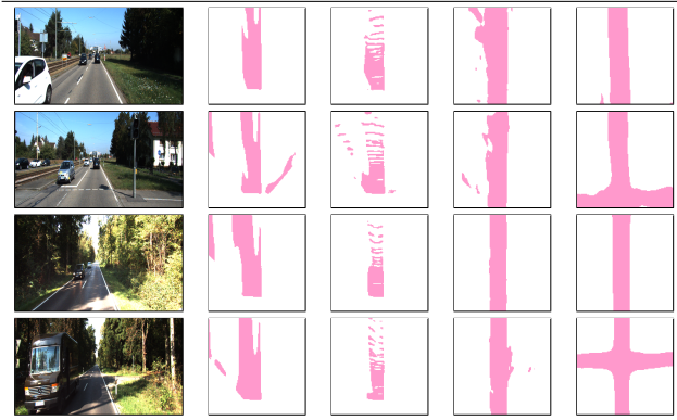
Figure 5: Impact of sensor fusion: Col 1: Input images. Col 2: Using per-frame monocular depth, Col 3: Using per-frame lidar depth, Col 4: Sensor-fused monocular depth, Col 5: Sensor-fused lidar depth. (Refer to Table 2 and Sec. 4.6 for more details)
