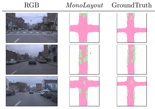
Figure 6: Amodal scene layout estimation on the Argoverse [3] dataset. The dataset comprises multiple challenging scenarios, with low illumination, large number of vehicles. MonoLayout is accurately able to produce sharp estimates of vehicles and road layouts. (Sidewalks are not predicted here, as they aren’t annotated in Argoverse).
