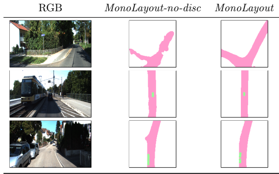
Figure 7: Effect of adversarial learning : As can be clearly seen here, the discriminators help enhance both the static (road) layout estimation (top and middle rows), as well as produce sharper vehicle boundaries (bottom row). While this translates to performance gains in static layout estimation ( c.f. Table 3), the gains in dynamic layout estimation are more cosmetic in nature.
