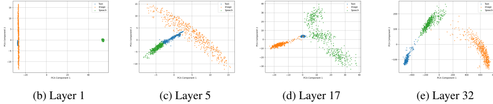
Figure 4: Multi-modal foundation model architecture and feature space analysis. a , Typical multi-modal foundation model processing interleaved text (T) and image (I) tokens (e.g., Chameleon (Chameleon Team, 2024)). Image tokens are derived from a pre-trained VQGAN model, converting an image into 1,024 discrete tokens. b , Principal Component Analysis of latent feature space for Chameleon+Speech 7B Dense model across layers 1, 5, 17, and 32. † Despite the model’s architecture processing all inputs as uniform discrete tokens without modality-specific priors, distinct clustering by modality (text, speech, image) is observed in the feature space. This natural clustering highlights the inherent differences between modalities, suggesting that the model might have processed them differently.
