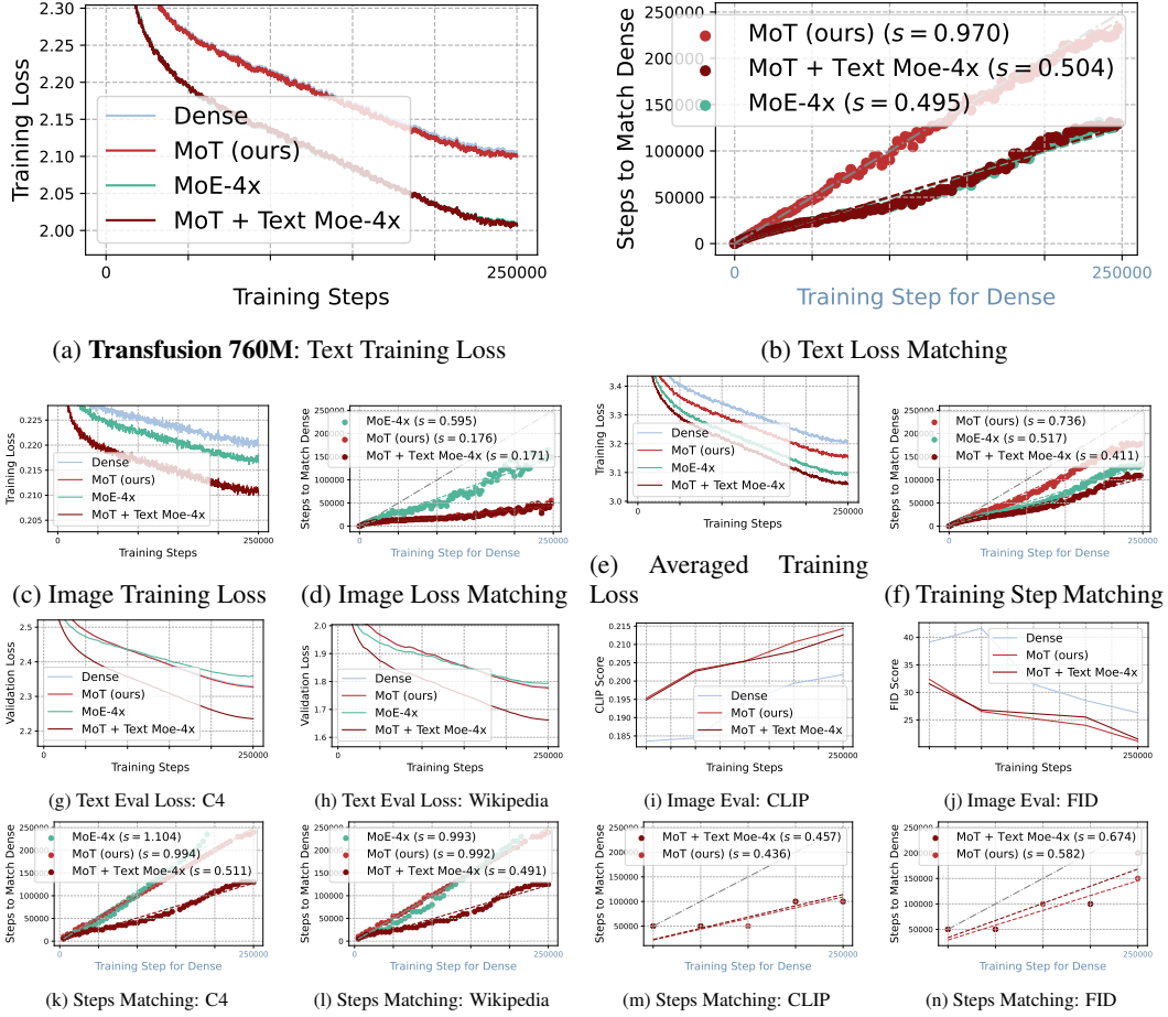
Figure 17: Combining MoT and MoE-4x in the Transfusion setting. a,b, Text training loss reduction significantly accelerated compared to dense model and MoT. c,d, Image modality performance benefits of MoT retained. e,f, Averaged training loss across both modalities. g-n, Validation losses on multiple representative text-only datasets and image generation evaluation results: "MoT + Text MoE-4x" achieves best text performance while maintaining comparable or slightly improved image performance relative to MoT. Both significantly outperform dense model and MoE-4x. MoE-4x shows better text training loss than dense model (a,b) but minimal improvement in text validation losses (g-h, k-l).
