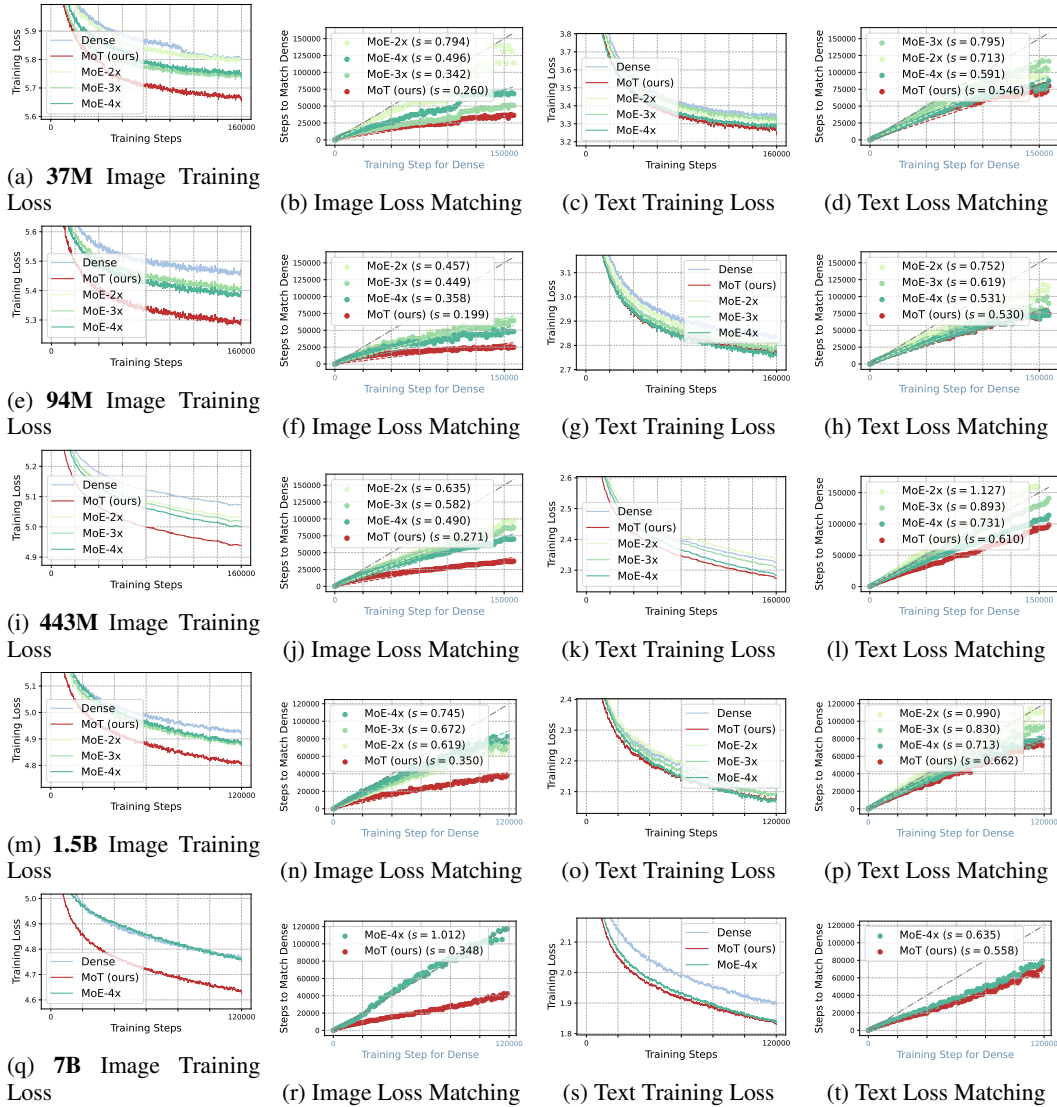
Figure 3: Modality-specific pre-training loss and step matching plots across model scales (Chameleon setting). MoT shows consistent, significant speedup in image modality across all scales (37M, 94M, 443M, 1.5B, 7B), outperforming dense and MoE-4x models. MoE-4x exhibits diminishing gains in image modality as scale increases, with advantages disappearing at 7B. In text modality, both MoT and MoE-4x outperform dense model, with MoT showing comparable or slightly better gains. Validation loss results in Appendix Figure 24). Model sizes for sparse models indicate activated parameters. All runs are FLOPs-controlled and pre-trained from scratch.
