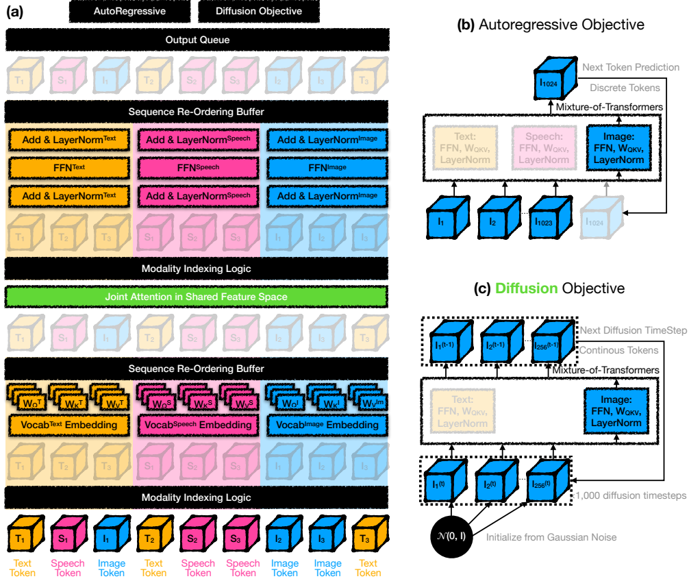
Figure 5: Mixture-of-Transformers architecture for multi-modal generative AI. a: Schematic of the sparsely activated Mixture-of-Transformers (MoT) architecture. For each input token, MoT activates modality-specific weights (including feed-forward networks, attention projection matrices, and layer normalization), then applies self-attention across the entire sequence. T , S , and I indicate text, speech, and image tokens, respectively. b-c: Flexibility in modality representation and training objectives. Images can be represented as (b) a sequence of discrete tokens trained with an autoregressive objective (Chameleon setting) or (c) a sequence of continuous tokens trained with a diffusion objective (Transfusion setting). This allows integration of diverse learning tasks, such as autoregressive objectives for text and diffusion-based objectives for images.
