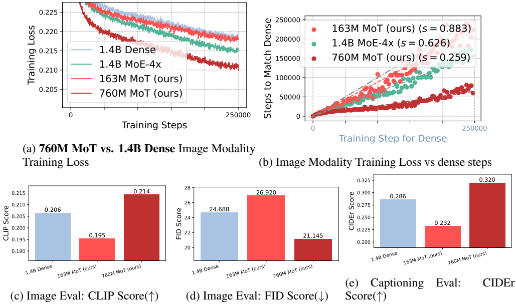
Figure 11: In the Transfusion setting, a 760M MoT model outperforms a 1.4B dense baseline across key image generation metrics, while using only half the FLOPs for both training and inference. a-b , MoT accelerates pre-training beyond Transfusion, particularly for image modality. The 760M MoT model, using half the training/inference FLOPs of the 1.4B dense baseline (Transfusion), consistently outperforms the dense model across metrics: CLIP score (0.214 vs 0.206, higher is better, (c) ), FID score (21.145 vs 24.688, lower is better, (d) ), CIDEr score for image captioning (0.320 vs 0.286, higher is better, (e) ), and image modality training loss. All runs are FLOPs-controlled and pre-trained from scratch, demonstrating MoT’s superior efficiency and performance across various model scales.
