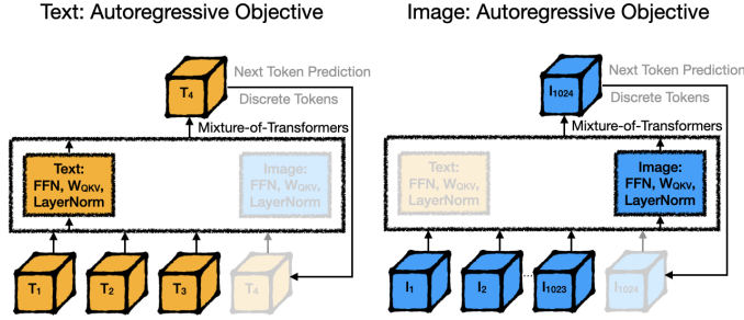
Figure 6: Multi-modal experiment setting with autoregressive objectives (Chameleon) . Both text and images are trained using autoregressive objectives. Images are tokenized into 1,024 discrete tokens using a pre-trained VQ-VAE model. This setting demonstrates unified processing across modalities with a single objective function.
