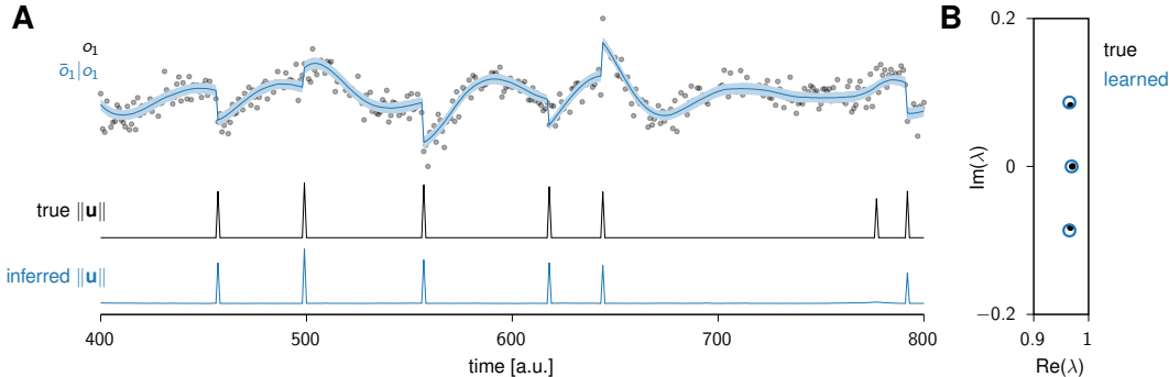
Figure 3: Inferring sparse inputs to a linear system. (A) Top: example observations (black dots) and inferred posterior mean (blue line). Bottom: true and inferred inputs. iLQR-VAE is able to infer the timing and magnitude of the inputs almost perfectly, despite being trained on only a single timeseries of 1000 time steps. Note that iLQR-VAE fails to infer one of the smallest inputs, whose effect on the observations is largely masked by observation noise. (B) Comparison of the true (black) and learned (blue) eigenvalue spectra. This shows that iLQR-VAE recovers the ground-truth dynamical system up to a similarity transformation.
