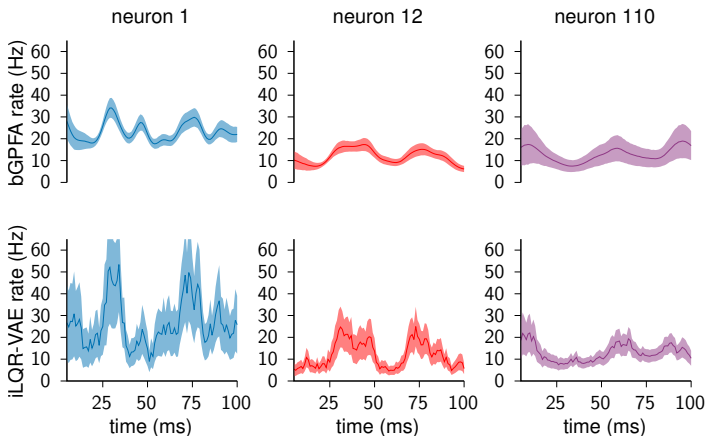
Figure S7: Comparison of the firing rates inferred by bGPFA and iLQR-VAE on the first 100ms of the continuous reaching task data, for three different neurons. bGPFA learns smoother trajectories. On the other hand, fitting iLQR-VAE with a Gaussian prior with no temporal structure allows to capture more variance in the firing rates, which in turn leads to a better decoding of the kinematics.
