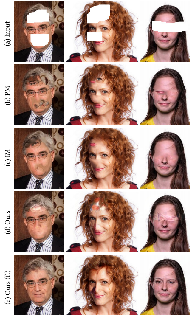
Fig. 15. Comparison with the PatchMatch (PM) and Image Melding (IM). We provide results for our general model (Ours), and our model fine-tuned for faces (Ours (ft)). Patch-based approaches are unable to generate novel objects in the scene leading to unnatural results. Photographs courtesy of Owen Lucas (Public Domain), Mon Mer (Public Domain), and SKV Floral (Public Domain). Additional results can be found in the supplemental materials.
