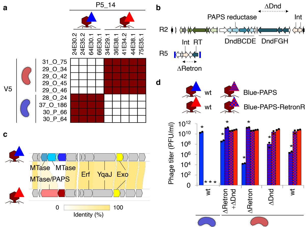
Figure 6. Bacterial defence and phage counter-defence.
