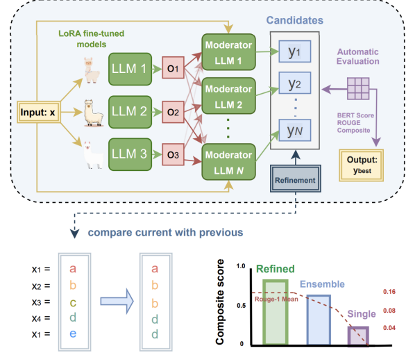
Figure 1: Overview of the proposed ensemble pipeline for inductive coding. The input x is processed by multiple LoRA fine-tuned models ( LLM_1, LLM_2, \dots, LLM_N ), generating candidate outputs ( O_1, O_2, \dots, O_N ). Moderators compare and evaluate these candidates, selecting y_1, y_2, \dots, y_N as refined candidates. Refinement of codes consists of comparing the current code with previous ones and assigning the same code based on the chosen similarity threshold.
