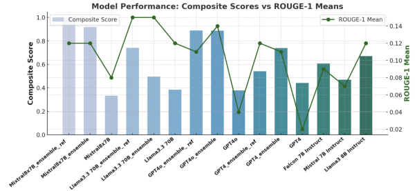
Figure 2: Performance comparison of different models on inductive coding tasks, measured by Composite Scores (bars) and ROUGE-1 Mean (line). Ensemble models with refinement outperform individual models and non-refinement ensembles.
