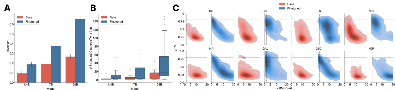
Figure 3. The ability to solve complex tasks increases with scale through alignment. ESM3 is aligned to follow tertiary coordination prompts with a dataset of preference pairs constructed from prompted generations, where positive samples with good scores for desired properties (high pTM, low cRMSD) are paired with negative samples with worse scores. The preference tuning loss encourages the model to put higher likelihood on the positive samples. After training, models are evaluated by prompting with the backbone atomic coordinates of residues in tertiary contact. (A) We show the effect of finetuning on the fraction of tasks solved with 128 generations (Pass@128; 2 s.d. error bars). A large gap opens between the models with scale. The response to alignment shows a latent capability to solve complex tasks in the largest model. (B) Number of distinct solutions (clustered at TM > 0.8) generated for each tertiary motif. After finetuning there are often many unique solutions for ligands where there are successes. (C) Densities of prompted generations are shown for the base model (left) and aligned model (right) at the 98B scale for a number of randomly selected ligands. After alignment, the fidelity to the prompt (backbone cRMSD) and quality of generations (pTM) tends to improve substantially.
