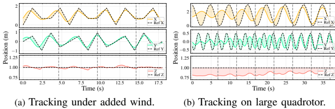
Fig. 4: Rapid policy adaptation using our proposed approach in the real world. Vertical dashed lines indicate policy update steps which occur every 5 s. Shaded regions represent the error from the reference.
