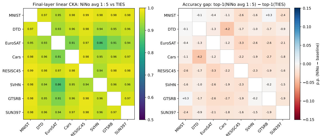
Figure 7. NiNo avg 1:5 against TIES. CKA remains high but the accuracy panel shifts more negative than the TA case, especially on DTD- and Cars-involving pairs.
