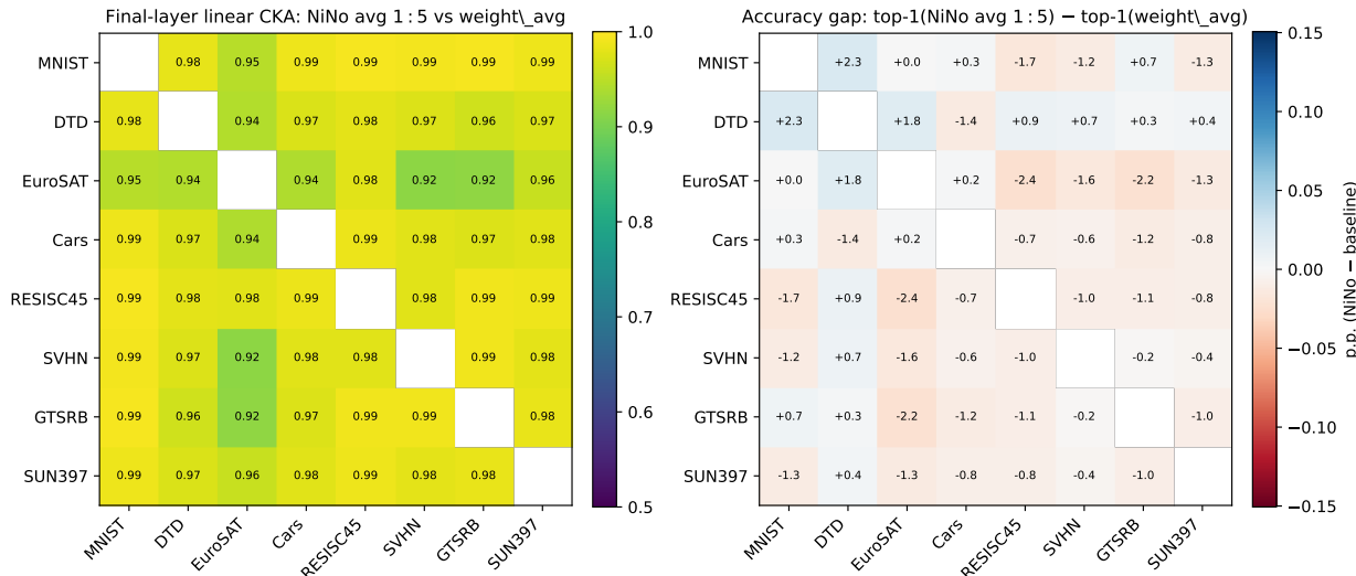
Figure 1. Per-pair 8x8 comparison of NiNo avg 1:5 against weight averaging. The left panel reports final-block linear CKA, averaged over the two in-pair evaluation datasets. The right panel reports the signed accuracy gap in percentage points. This is the closest baseline to NiNo in activation space on the 28-pair grid.
