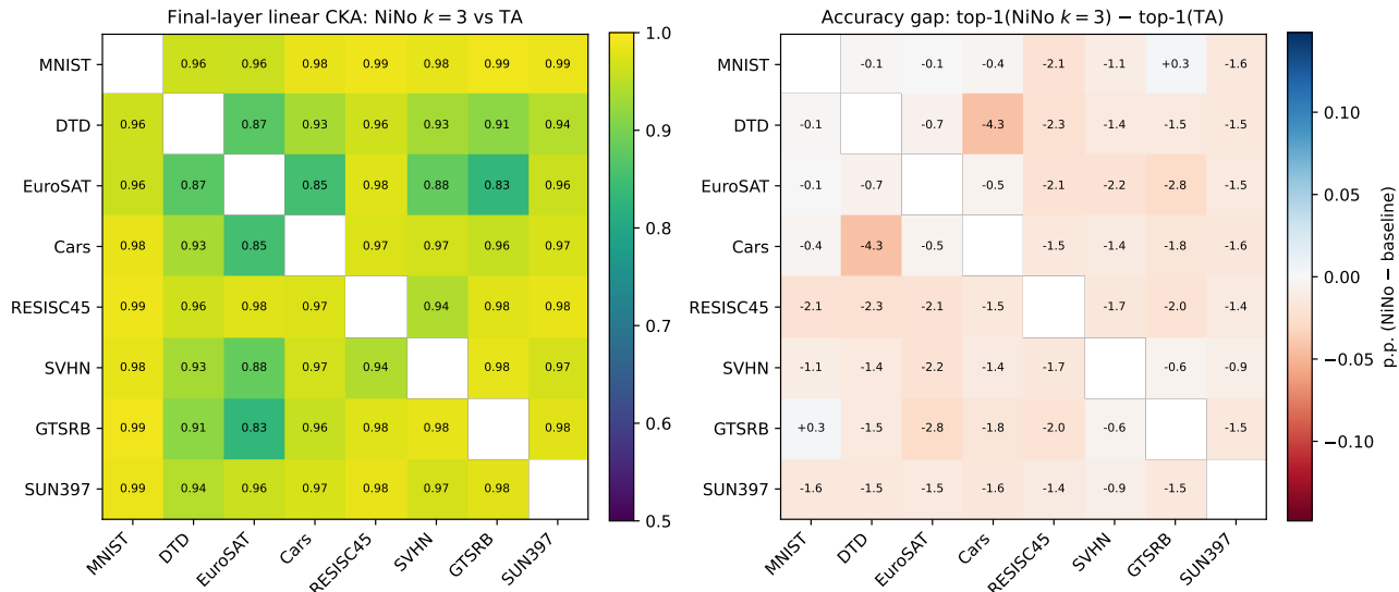
Figure 5. Per-pair 8 \times 8 comparison of NiNo k=3 against Task Arithmetic. Same construction as Figure 4, with the single best NiNo horizon ( k=3 ) as the anchor.
