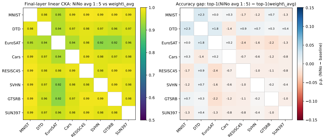
Figure 6. NiNo avg 1:5 against weight averaging. The CKA panel saturates above 0.95 on most pairs, confirming weight averaging as NiNo’s nearest baseline in activation space.
