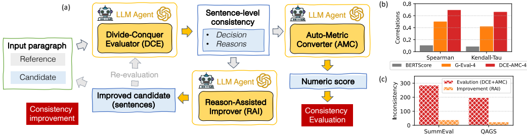
Figure 1: (a) Overview of the proposed DCR framework. The first two components (DCE-AMC) aim at providing a better strategy for evaluating and quantifying semantic consistency to best match human judgments. Building on this, a third component RAI further utilizes analytical reasoning to iteratively improve the consistency of LLM-generated content w.r.t. the reference by minimizing hallucinations. (b) The combination of DCE and AMC (DCE-AMC-4) significantly outperforms the baseline methods in terms of correlations with human ratings. (c) RAI substantially reduces output inconsistencies by \sim 90\% through a single improvement iteration on SummEval and QAGS benchmarks.
