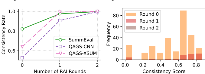
Figure 4: Multi-round consistency improvement
