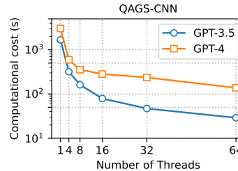
Figure 5: Computational cost.
