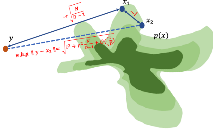
Figure 6. Illustration of the phase alignment analysis
