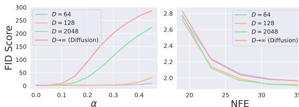
Figure 5. FID score versus (left) \alpha and (right) NFE on CIFAR-10.
