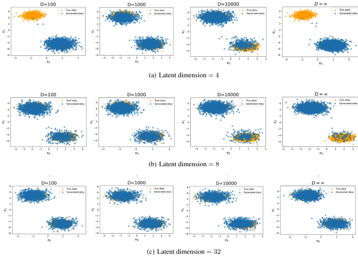
Figure 11. Visualization of the first two coordinates ( x_0, x_1 ) for the generated data (blue) versus true data (orange). From the top row to the bottom row: the latent dimension of the neural network is set to 4 (a), 8 (b), and 32 (c).
