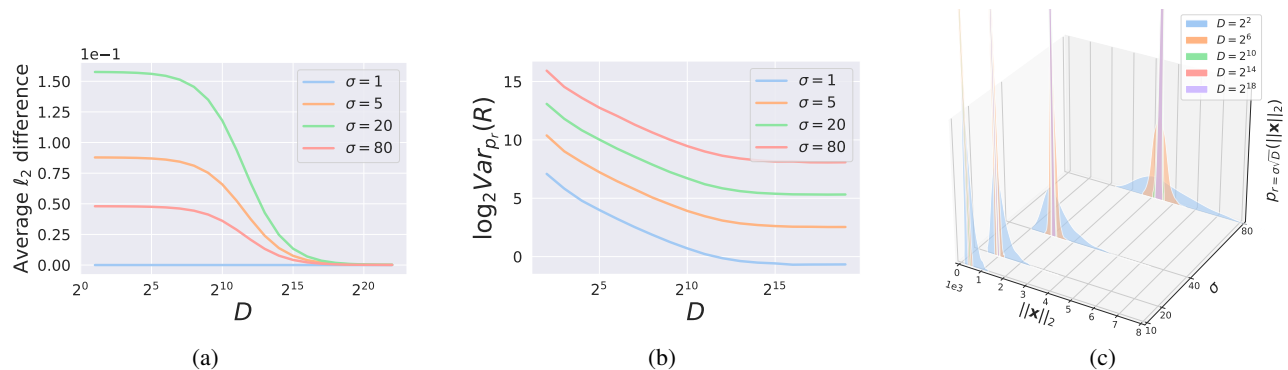
Figure 4. (a) Average l_2 difference between scaled electric field and score function, versus D . (b) Log-variance of radius distribution versus D . (c) Density of radius distributions p_{r=\sigma\sqrt{D}}(R) with varying \sigma and D .
