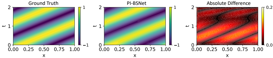
Figure 5: Test results on advection equations with unseen parameter.
