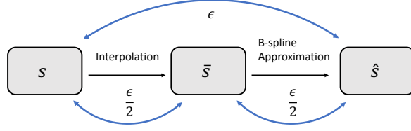
Figure 7: Relationships between ground truth s , interpolation \bar{s} , and B-spline approximation \hat{s} used in the proof of Lemma C.3.
