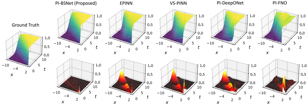
Figure 2: Recovery probability visualizations. Predictions in first row and errors in second row.
