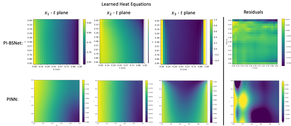
Figure 20: The learned solutions (left) and the residuals (right) for the 3D heat equations.
