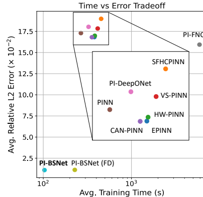
Figure 4: Training time vs. prediction error trade-offs.
