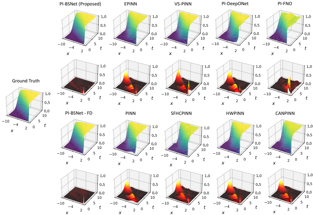
Figure 12: Recovery probability visualizations. Predictions in first row and errors in second row.
