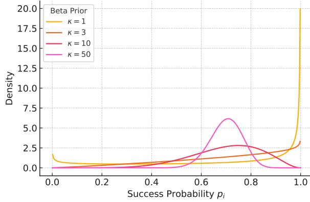
Figure 4: Effect of the concentration parameter \kappa on the Beta prior. All curves are plotted with fixed mean w_i = 0.7 . Larger \kappa yields a more concentrated prior around w_i , while smaller \kappa reflects greater uncertainty.
