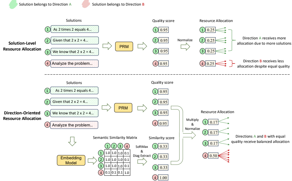
Figure 2: Comparison between Solution-Level Resource Allocation and proposed Direction-Oriented Resource Allocation (DORA).
