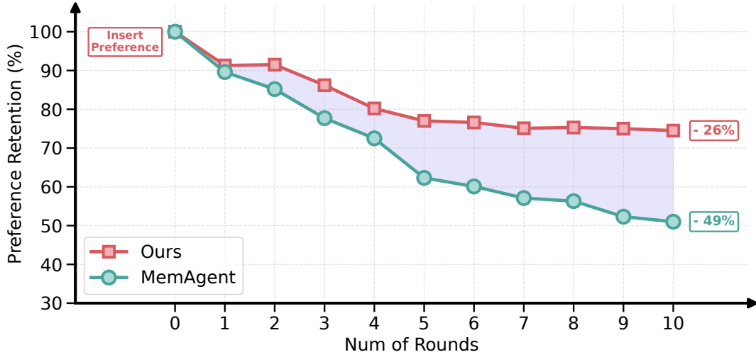
Figure 7: Preference retention over during multi-round memory evolution on PrefEval (Explicit). We insert a user preference at round 0 and then run memory evolution for subsequent rounds, where each round uses a 4K-token dialogue context. A strong judge model (Gemini-2.5-Pro) verifies whether the preference remains in the memory bank after each round.
