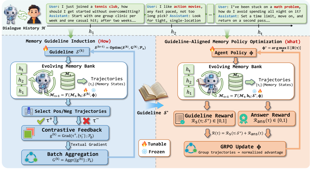
Figure 2: Overview of our proposed MemCoE . It performs two-stage optimization for evolving user memory: (1) Memory Guideline Induction (MGI) iteratively refines a natural-language guideline; (2) Guideline-Aligned Memory Policy Optimization (GMPO) fixes the induced guideline to define guideline-aligned rewards and applies multi-turn GRPO to learn what information to update in evolving memory bank.
