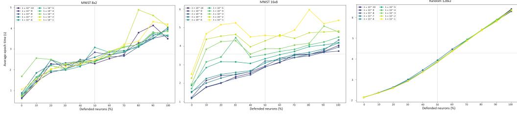
Figure 5: Training overhead of similarity regularization across different architectures. Average training time per epoch versus percentage of defended neurons for (left) MNIST 8 \times 2, (center) MNIST 16 \times 8, and (right) Random 128 \times 2 architectures with varying \lambda_{similarity} values. Baseline training times (0% defense) are 0.65s, 0.83s, and 1.37s respectively. As the percentage of defended neurons increases, training time scales approximately linearly, reaching ranges of [0.98s–3.73s], [1.2s–4.3s], and [2.05s–6.93s]. The computational overhead stems from pairwise neuron comparisons, which scale with both network size and the fraction of defended neurons.
