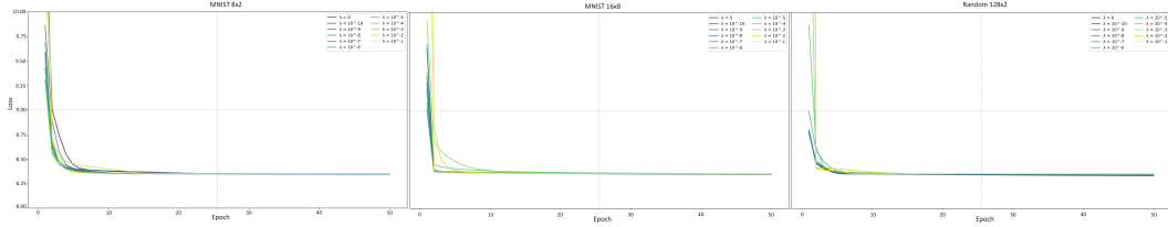
Figure 6: Training loss across epochs for different regularization strengths ( \lambda_{similarity} ) on three architectures: MNIST 8 \times 2, MNIST 16 \times 8, and Random 128 \times 2. Across all models, the similarity regularizer causes minimal variation in convergence behavior, with all curves stabilizing within roughly five epochs of the baseline ( \lambda = 0 ).
