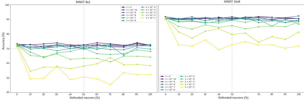
Figure 4: Impact of similarity regularization on model accuracy across different architectures. Accuracy versus percentage of defended neurons for (left) 8×2 and (right) 16×8 architectures on MNIST, with varying \lambda_{\text{similarity}} values. The baseline ( \lambda_{\text{similarity}} = 0 ) maintains stable accuracy around 72.7% and 90.7% for 8×2 and 16×8 respectively. Small lambda values ( \lambda_{\text{similarity}} \leq 10^{-7} ) show minimal accuracy degradation, while larger values progressively reduce accuracy. The 16×8 architecture demonstrates greater robustness to regularization, maintaining higher accuracy even at larger \lambda_{\text{similarity}} values.
