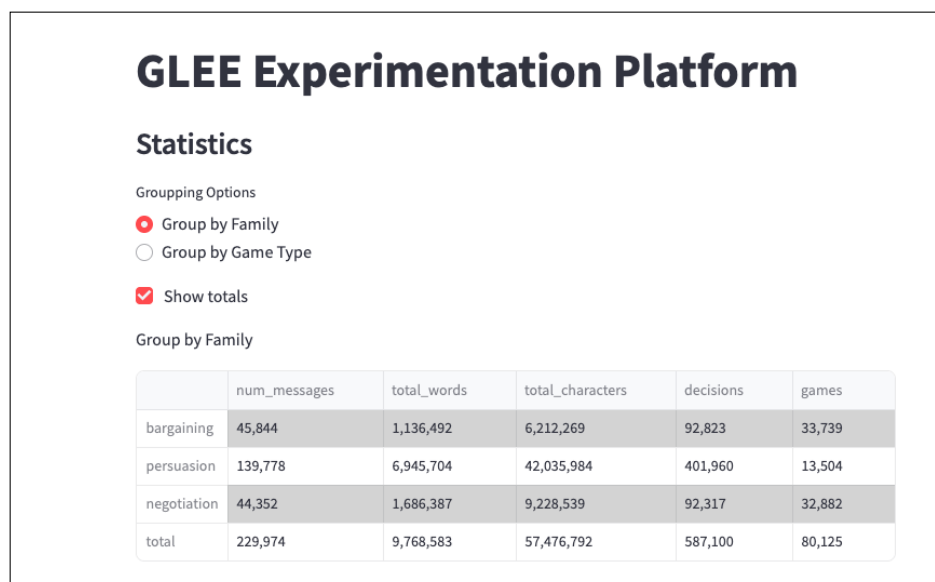
Figure 7: Data analysis: Statistics table summarizing key characteristics of the collected data.
