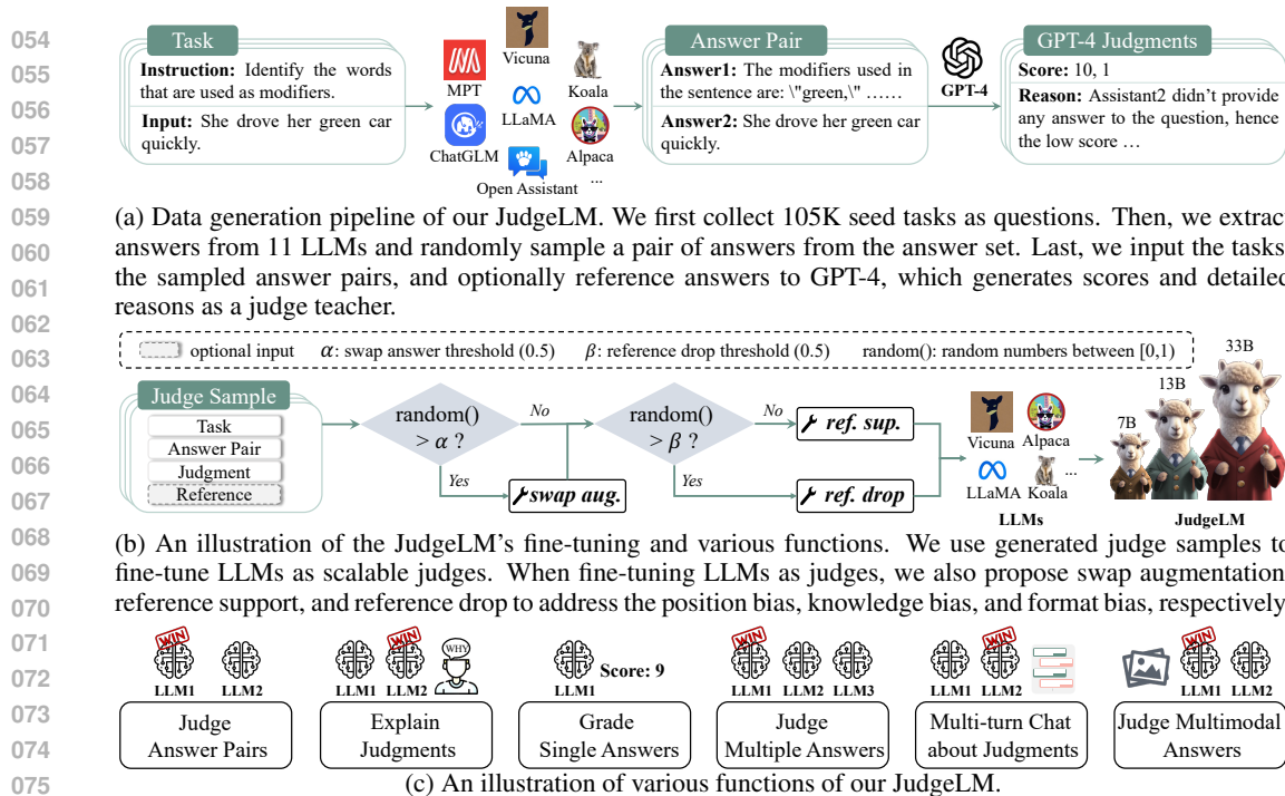
Figure 1: An overview of our scalable JudgeLM including data generation, fine-tuning, and various functions.
