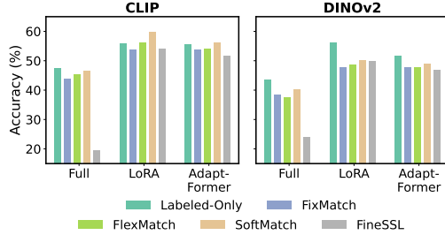
Figure 3: Average SSL accuracy with full fine-tuning or PEFT across 12 settings shows that, with fair hyper-parameter tuning, fine-tuning on limited labels can outperform SSL; PEFT boosts SSL yet matches labeled-only performance, indicating minimal unlabeled-data benefit in current VFM-based SSL (see appendix B.3).
