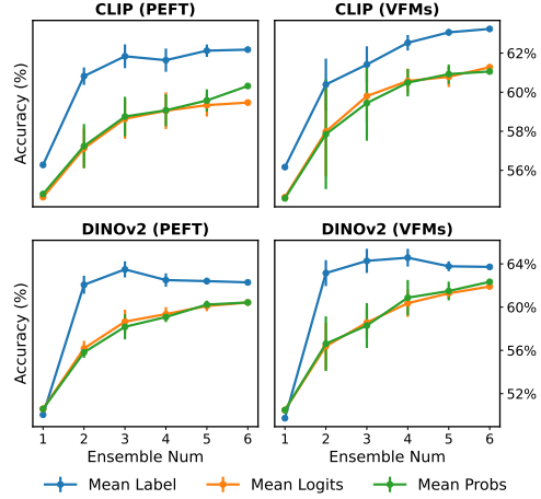
Figure 6: Scaling analysis for ensembling more PEFT methods and VFMs. Starting from LoRA fine-tuning, performance improves with diverse pseudo-labels, but the gain diminishes with more ensemble sources. Mean Label consistently outperforms Mean Logits and Mean Probabilities .
