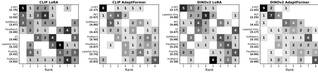
Figure 5: Ranking frequency across SSL methods by the proposed benchmark. The number in (i, j) indicates the frequency of method i is ranked j -th across 12 settings. The number in brackets indicates the average rank, where the higher rank is better.
